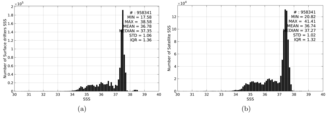
Figure 2: Histograms of SSS from Surface drifters (a) and SMOS-L3-CATDS-CECOS-LOCEAN-V2-18DAYS-25KM (b) considering all match-up pairs per bins of 0.1 over the Mid-Low Latitudes 45N-45S Pi-MEP region and for the full satellite product period.
