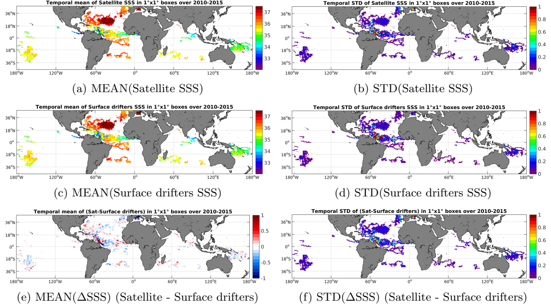
Figure 5: Temporal mean (left) and STD (right) of SSS from SMOS-L3-CATDS-CECOS-LOCEAN-V2-18DAYS-25KM (top), Surface drifters (middle), and of \Delta SSS (Satellite - Surface drifters). Only match-up pairs are used to generate these maps.
