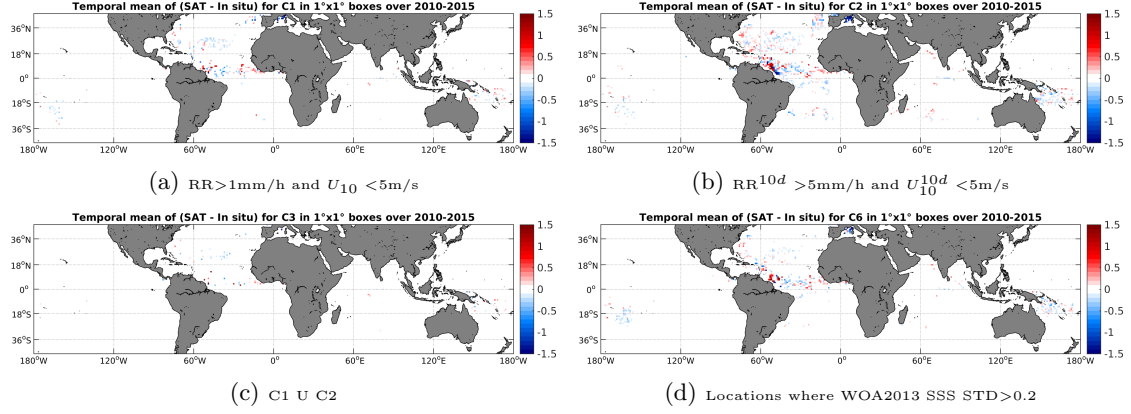
Figure 11: Temporal mean gridded over spatial boxes of size 1^\circ \times 1^\circ of \Delta SSS (SMOS-L3-CATDS-CECOS-LOCEAN-V2-18DAYS-25KM - Surface drifters) for 4 different subdatasets corresponding to: RR > 1\text{mm/h} and U_{10} < 5\text{m/s} (a), RR^{10d} > 5\text{mm/h} and U_{10}^{10d} < 5\text{m/s} (b), C1 U C2 (c), Locations where WOA2013 SSS STD > 0.2 (d).
