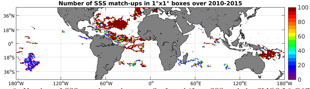
Figure 3: Number of SSS match-ups between Surface drifters SSS and the SMOS-L3-CATDS-CECOS-LOCEAN-V2-18DAYS-25KM SSS product for the Mid-Low Latitudes 45N-45S Pi-MEP region over 1°x1° boxes and for the full satellite product period.
