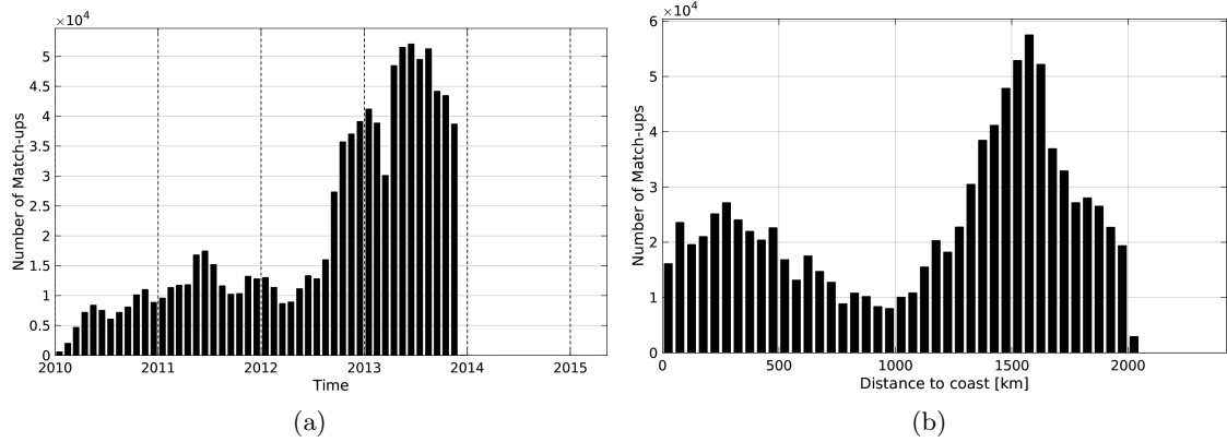
Figure 1: Number of match-ups between Surface drifters and SMOS-L3-CATDS-CECOS-LOCEAN-V2-18DAYS-25KM SSS as a function of time (a) and as function of the distance to coast (b) over the Mid-Low Latitudes 45N-45S Pi-MEP region and for the full satellite product period.
