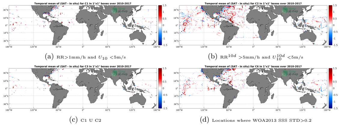
Figure 12: Temporal mean gridded over spatial boxes of size 1^\circ \times 1^\circ of \Delta SSS (SMOS-L3-CATDS-IFREMER-CECOS-V2-MONTHLY-0.25DEG - TSG-SAMOS) for 4 different subdatasets corresponding to: RR > 1\text{mm/h} and U_{10} < 5\text{m/s} (a), RR^{10d} > 5\text{mm/h} and U_{10}^{10d} < 5\text{m/s} (b), C1 U C2 (c), Locations where WOA2013 SSS STD > 0.2 (d).
