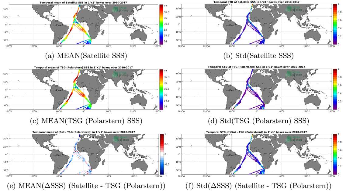
Figure 6: Temporal mean (left) and Std (right) of SSS from SMOS SSS L3 v2 - Monthly - 0.25 Deg (CATDS-CECOS-IFREMER) (top), TSG (Polarstern) (middle), and of \Delta SSS (Satellite - TSG (Polarstern)). Only match-up pairs are used to generate these maps.
