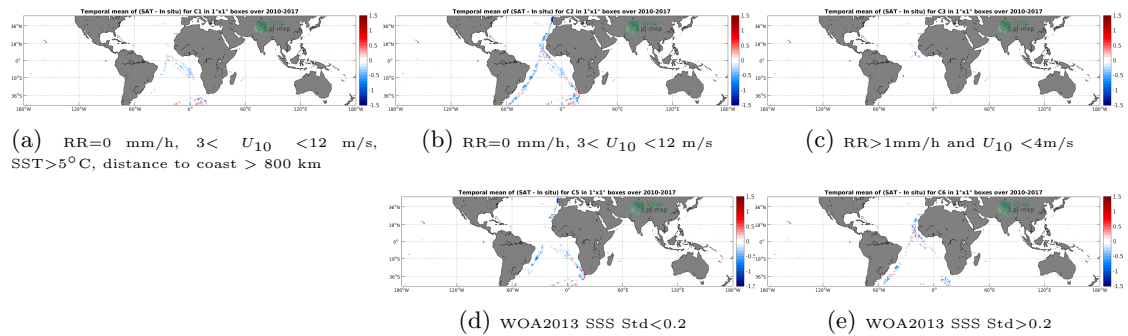
Figure 12: Temporal mean gridded over spatial boxes of size 1^\circ \times 1^\circ of \Delta SSS (SMOS L3 v2 - Monthly - 0.25 Deg (CATDS-CECOS-IFREMER) - TSG-POLARSTERN) for 5 different sub-datasets corresponding to:RR=0 mm/h, 3 < U_{10} < 12 m/s, SST > 5^\circ\text{C} , distance to coast > 800 km (a), RR=0 mm/h, 3 < U_{10} < 12 m/s (b), RR > 1 mm/h and U_{10} < 4 m/s (c), WOA2013 SSS Std < 0.2 (d), WOA2013 SSS Std > 0.2 (e).
