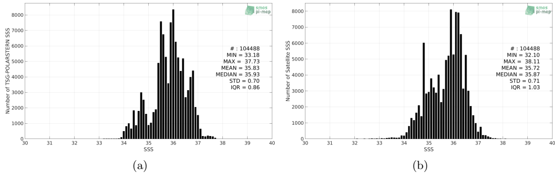
Figure 2: Histograms of SSS from TSG-POLARSTERN (a) and SMOS L3 v2 - Monthly - 0.25 Deg (CATDS-CECOS-IFREMER) (b) considering all match-up pairs per bins of 0.1 over the Mid-Low Latitudes 45N-45S Pi-MEP region and for the full satellite product period.
