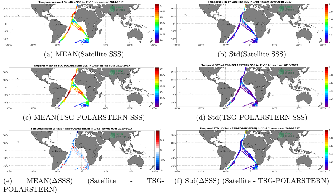
Figure 6: Temporal mean (left) and Std (right) of SSS from SMOS L3 v2 - Monthly - 0.25 Deg (CATDS-CECOS-IFREMER) (top), TSG-POLARSTERN (middle), and of \Delta SSS (Satellite - TSG-POLARSTERN). Only match-up pairs are used to generate these maps.
