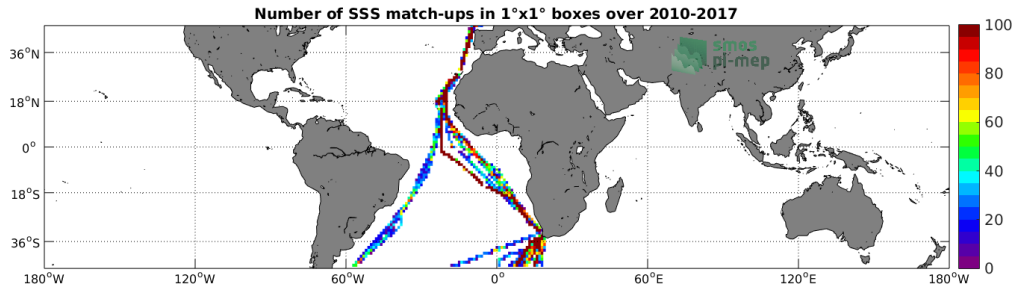
Figure 4: Number of SSS match-ups between TSG-POLARSTERN SSS and the SMOS L3 v2 - Monthly - 0.25 Deg (CATDS-CECOS-IFREMER) SSS product for the Mid-Low Latitudes 45N-45S Pi-MEP region over 1°x1° boxes and for the full satellite product period.
