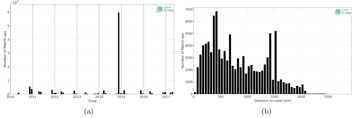
Figure 1: Number of match-ups between TSG-POLARSTERN and SMOS L3 v2 - Monthly - 0.25 Deg (CATDS-CECOS-IFREMER) SSS as a function of time (a) and as function of the distance to coast (b) over the Mid-Low Latitudes 45N-45S Pi-MEP region and for the full satellite product period.
