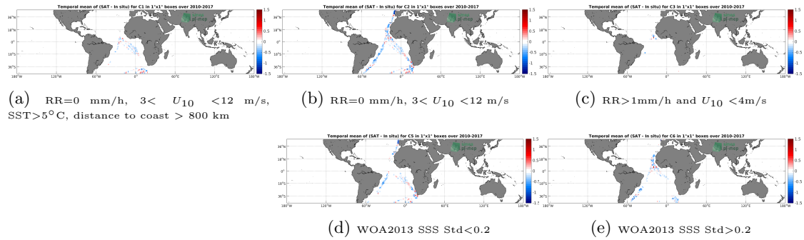
Figure 12: Temporal mean gridded over spatial boxes of size 1^\circ \times 1^\circ of \Delta SSS (SMOS-L3-CATDS-IFREMER-CECOS-V2-MONTHLY-0.25DEG - TSG-POLARSTERN) for 5 different subdatasets corresponding to:RR=0 mm/h, 3 < U_{10} < 12 m/s, SST > 5^\circ\text{C} , distance to coast > 800 km (a), RR=0 mm/h, 3 < U_{10} < 12 m/s (b), RR > 1 mm/h and U_{10} < 4 m/s (c), WOA2013 SSS Std < 0.2 (d), WOA2013 SSS Std > 0.2 (e).
