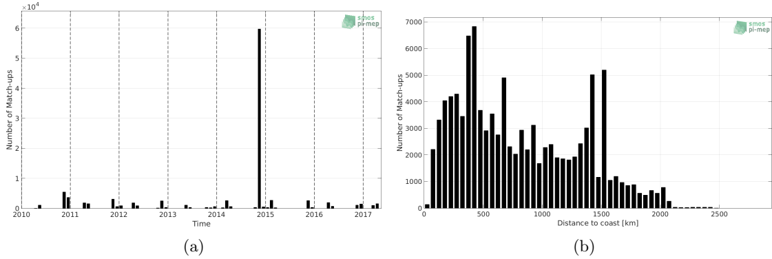
Figure 1: Number of match-ups between TSG-POLARSTERN and SMOS-L3-CATDS-IFREMER-CECOS-V2-MONTHLY-0.25DEG SSS as a function of time (a) and as function of the distance to coast (b) over the Mid-Low Latitudes 45N-45S Pi-MEP region and for the full satellite product period.
