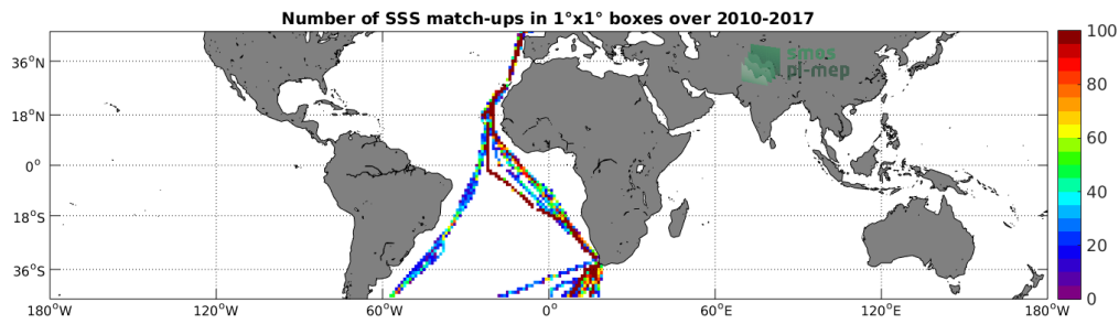
Figure 4: Number of SSS match-ups between TSG-POLARSTERN SSS and the SMOS-L3-CATDS-IFREMER-CECOS-V2-MONTHLY-0.25DEG SSS product for the Mid-Low Latitudes 45N-45S Pi-MEP region over 1^\circ \times 1^\circ boxes and for the full satellite product period.
