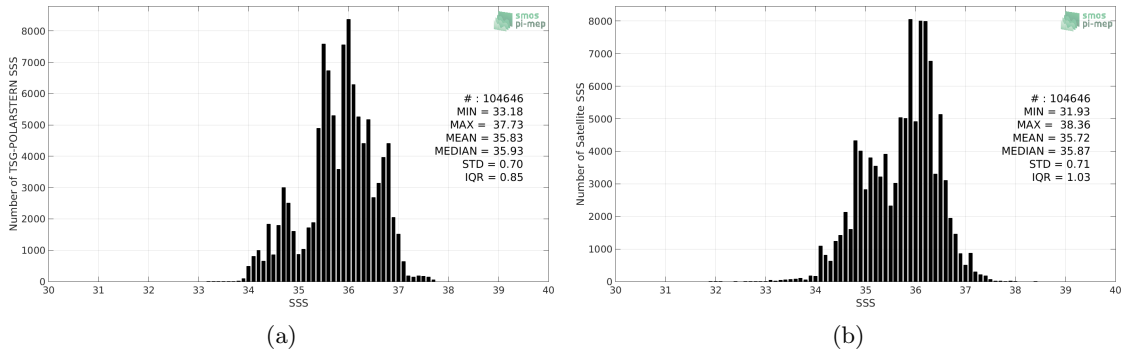
Figure 2: Histograms of SSS from TSG-POLARSTERN (a) and SMOS-L3-CATDS-IFREMER-CECOS-V2-MONTHLY-0.25DEG (b) considering all match-up pairs per bins of 0.1 over the Mid-Low Latitudes 45N-45S Pi-MEP region and for the full satellite product period.
