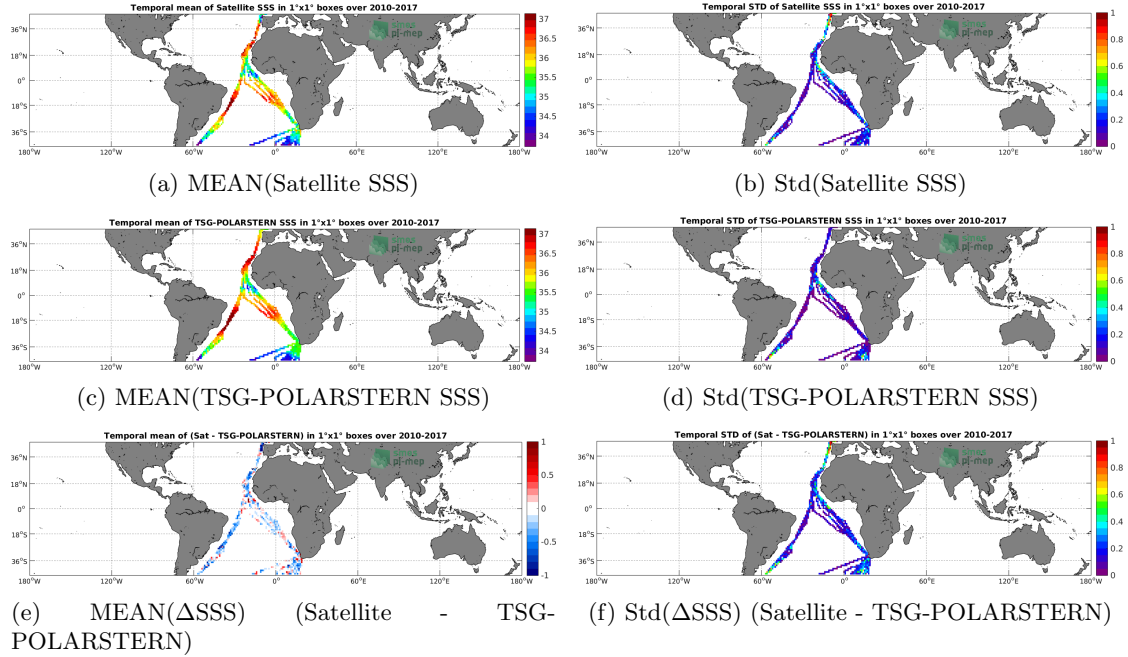
Figure 6: Temporal mean (left) and Std (right) of SSS from SMOS-L3-CATDS-IFREMER-CECOS-V2-MONTHLY-0.25DEG (top), TSG-POLARSTERN (middle), and of \Delta SSS (Satellite - TSG-POLARSTERN). Only match-up pairs are used to generate these maps.
