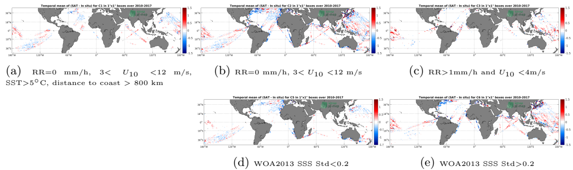
Figure 12: Temporal mean gridded over spatial boxes of size 1^\circ \times 1^\circ of \Delta SSS (SMOS L3 v2 - Monthly - 0.25 Deg (CATDS-CECOS-IFREMER) - TSG-LEGOS-DM) for 5 different subdatasets corresponding to: RR=0 mm/h, 3 < U_{10} < 12 m/s, SST > 5^\circ C , distance to coast > 800 km (a), RR=0 mm/h, 3 < U_{10} < 12 m/s (b), RR > 1 mm/h and U_{10} < 4 m/s (c), WOA2013 SSS Std < 0.2 (d), WOA2013 SSS Std > 0.2 (e).
