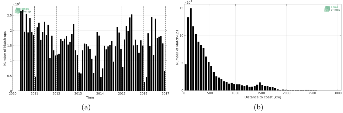
Figure 1: Number of match-ups between TSG-LEGOS-DM and SMOS-L3-CATDS-IFREMER-CECOS-V2-MONTHLY-0.25DEG SSS as a function of time (a) and as function of the distance to coast (b) over the Mid-Low Latitudes 45N-45S Pi-MEP region and for the full satellite product period.
