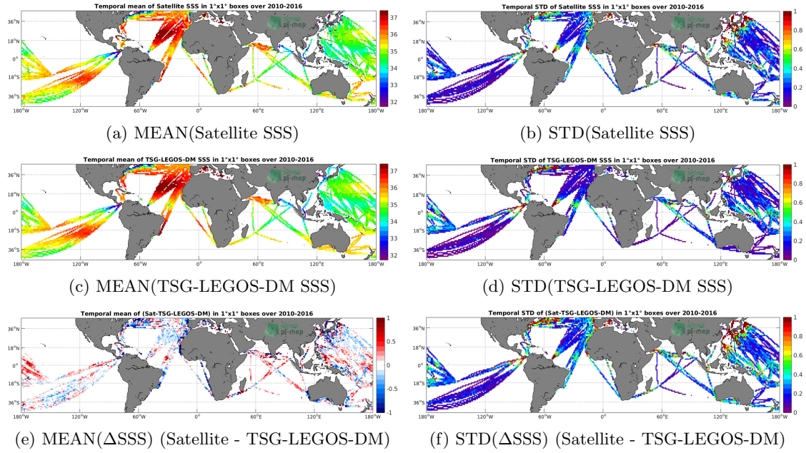
Figure 6: Temporal mean (left) and STD (right) of SSS from SMOS-L3-CATDS-IFREMER-CECOS-V2-MONTHLY-0.25DEG (top), TSG-LEGOS-DM (middle), and of \Delta SSS (Satellite - TSG-LEGOS-DM). Only match-up pairs are used to generate these maps.
