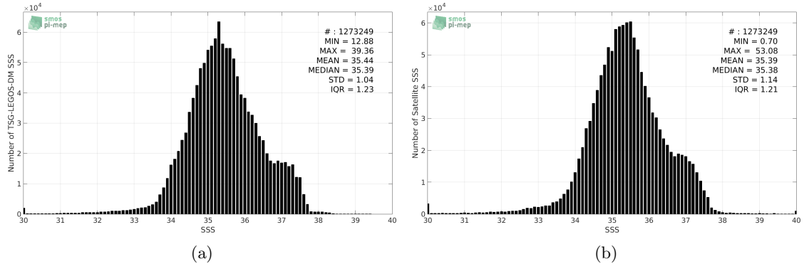
Figure 2: Histograms of SSS from TSG-LEGOS-DM (a) and SMOS-L3-CATDS-IFREMER-CECOS-V2-MONTHLY-0.25DEG (b) considering all match-up pairs per bins of 0.1 over the Mid-Low Latitudes 45N-45S Pi-MEP region and for the full satellite product period.
