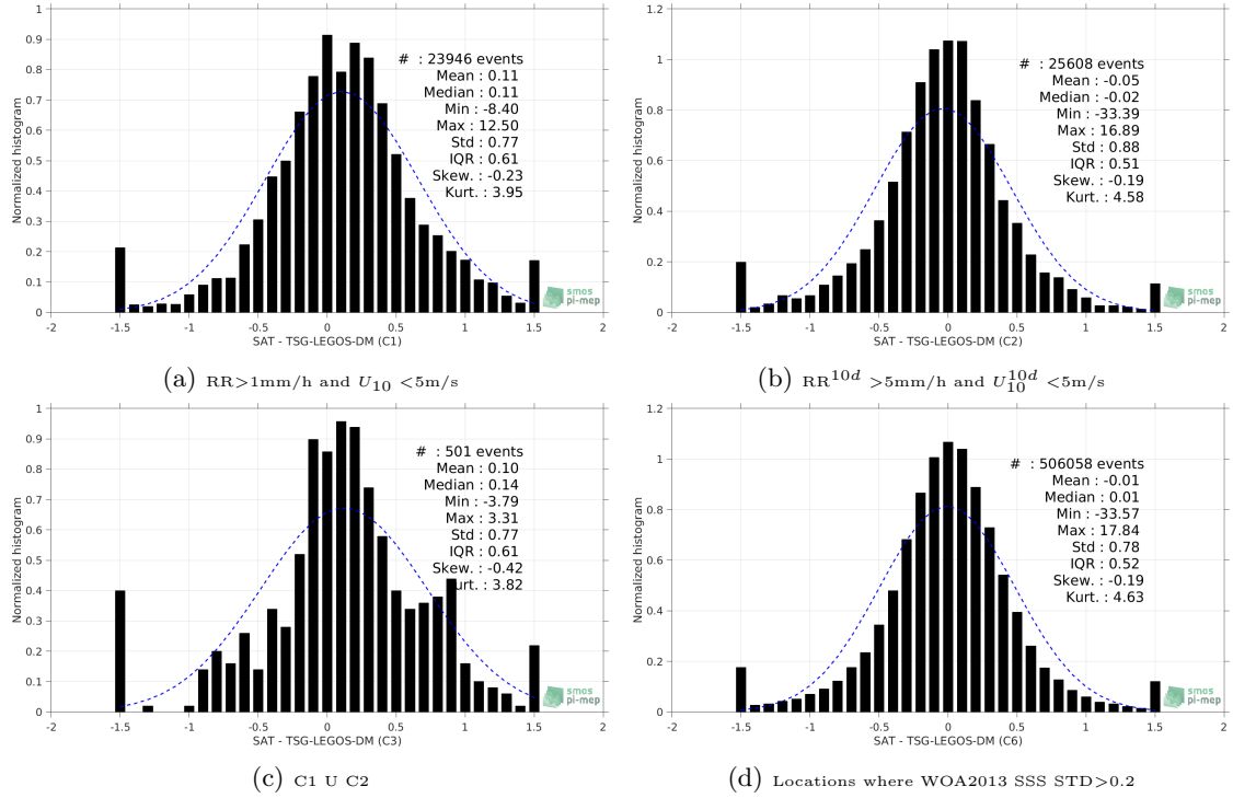
Figure 13: Normalized histogram of \Delta SSS (SMOS-L3-CATDS-IFREMER-CECOS-V2-MONTHLY-0.25DEG - TSG-LEGOS-DM) for 6 different subdatasets corresponding to: RR > 1\text{mm/h} and U_{10} < 5\text{m/s} (a), RR^{10d} > 5\text{mm/h} and U_{10}^{10d} < 5\text{m/s} (b), C1 U C2 (c), Locations where WOA2013 SSS STD > 0.2 (d).
