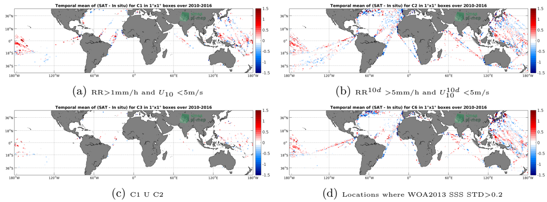
Figure 12: Temporal mean gridded over spatial boxes of size 1^\circ \times 1^\circ of \Delta SSS (SMOS-L3-CATDS-IFREMER-CECOS-V2-MONTHLY-0.25DEG - TSG-LEGOS-DM) for 4 different subdatasets corresponding to: RR > 1\text{mm/h} and U_{10} < 5\text{m/s} (a), RR^{10d} > 5\text{mm/h} and U_{10}^{10d} < 5\text{m/s} (b), C1 U C2 (c), Locations where WOA2013 SSS STD > 0.2 (d).
