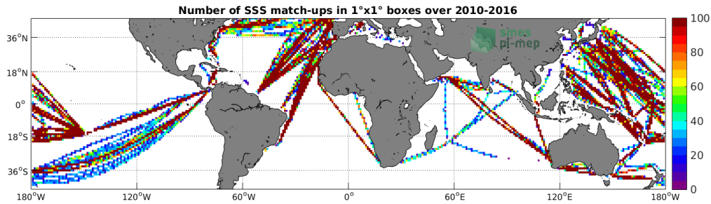
Figure 4: Number of SSS match-ups between TSG-LEGOS-DM SSS and the SMOS-L3-CATDS-IFREMER-CECOS-V2-MONTHLY-0.25DEG SSS product for the Mid-Low Latitudes 45N-45S Pi-MEP region over 1^\circ \times 1^\circ boxes and for the full satellite product period.
