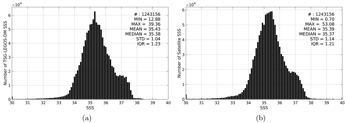
Figure 2: Histograms of SSS from TSG-LEGOS-DM (a) and SMOS-L3-CATDS-IFREMER-CECOS-V2-MONTHLY-0.25DEG (b) considering all match-up pairs per bins of 0.1 over the Mid-Low Latitudes 45N-45S Pi-MEP region and for the full satellite product period.
