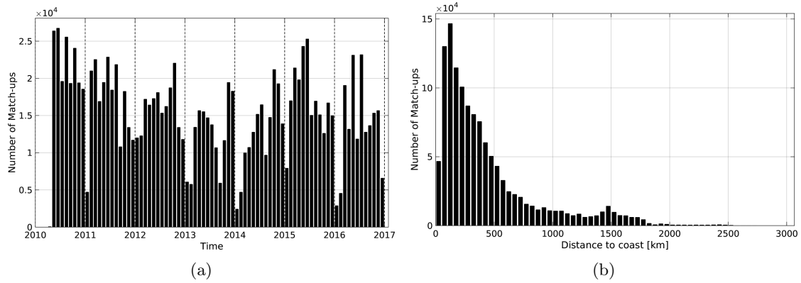
Figure 1: Number of match-ups between TSG-LEGOS-DM and SMOS-L3-CATDS-IFREMER-CECOS-V2-MONTHLY-0.25DEG SSS as a function of time (a) and as function of the distance to coast (b) over the Mid-Low Latitudes 45N-45S Pi-MEP region and for the full satellite product period.
