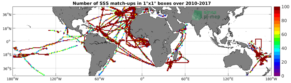
Figure 4: Number of SSS match-ups between TSG (GOSUD-Research-vessel) SSS and the SMOS SSS L3 v2 - Monthly - 0.25 Deg (CATDS-CECOS-IFREMER) SSS product for the Mid-Low Latitudes 45N-45S Pi-MEP region over 1°x1° boxes and for the full satellite product period.
