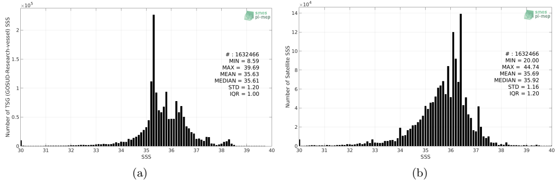
Figure 2: Histograms of SSS from TSG (GOSUD-Research-vessel) (a) and SMOS SSS L3 v2 - Monthly - 0.25 Deg (CATDS-CECOS-IFREMER) (b) considering all match-up pairs per bins of 0.1 over the Mid-Low Latitudes 45N-45S Pi-MEP region and for the full satellite product period.
