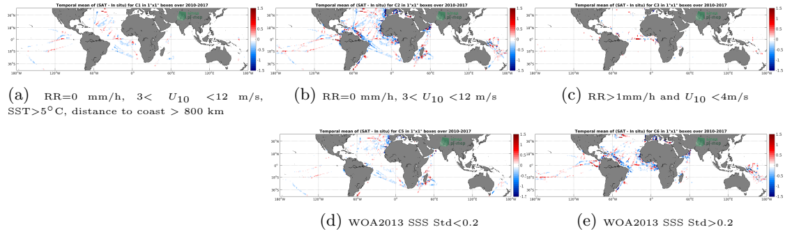
Figure 12: Temporal mean gridded over spatial boxes of size 1^\circ \times 1^\circ of \Delta SSS (SMOS SSS L3 v2 - Monthly - 0.25 Deg (CATDS-CECOS-IFREMER) - TSG (GOSUD-Research-vessel)) for 5 different subdatasets corresponding to: RR=0 mm/h, 3 < U_{10} < 12 m/s, SST > 5^\circ C , distance to coast > 800 km (a), RR=0 mm/h, 3 < U_{10} < 12 m/s (b), RR > 1 mm/h and U_{10} < 4 m/s (c), WOA2013 SSS Std < 0.2 (d), WOA2013 SSS Std > 0.2 (e).
