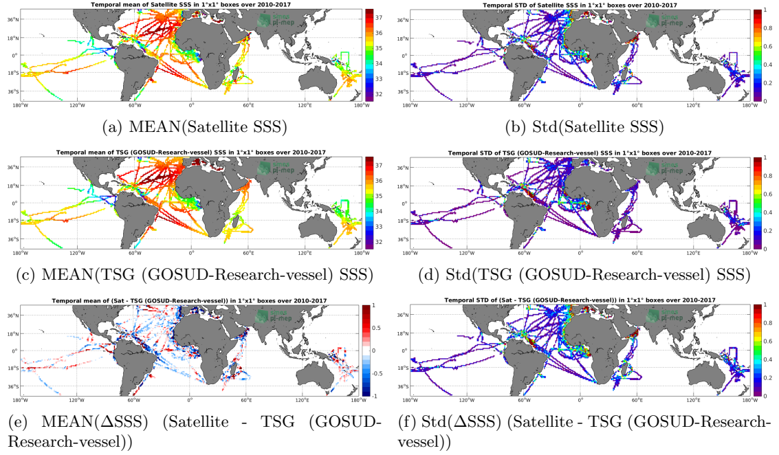
Figure 6: Temporal mean (left) and Std (right) of SSS from SMOS SSS L3 v2 - Monthly - 0.25 Deg (CATDS-CECOS-IFREMER) (top), TSG (GOSUD-Research-vessel) (middle), and of \Delta SSS (Satellite - TSG (GOSUD-Research-vessel)). Only match-up pairs are used to generate these maps.
