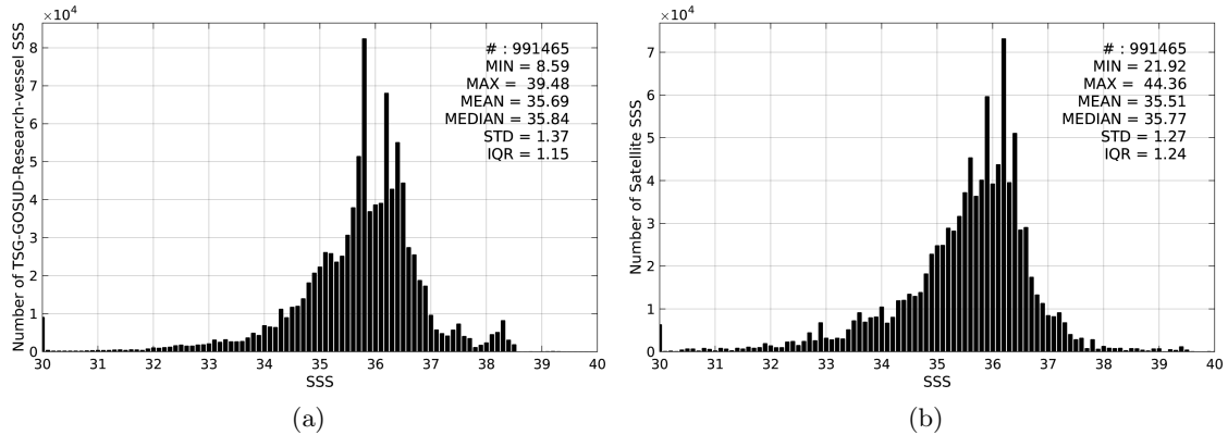
Figure 2: Histograms of SSS from TSG-GOSUD-Research-vessel (a) and SMOS-L3-CATDS-IFREMER-CECOS-V2-MONTHLY-0.25DEG (b) considering all match-up pairs per bins of 0.1 over the Mid-Low Latitudes 45N-45S Pi-MEP region and for the full satellite product period.
