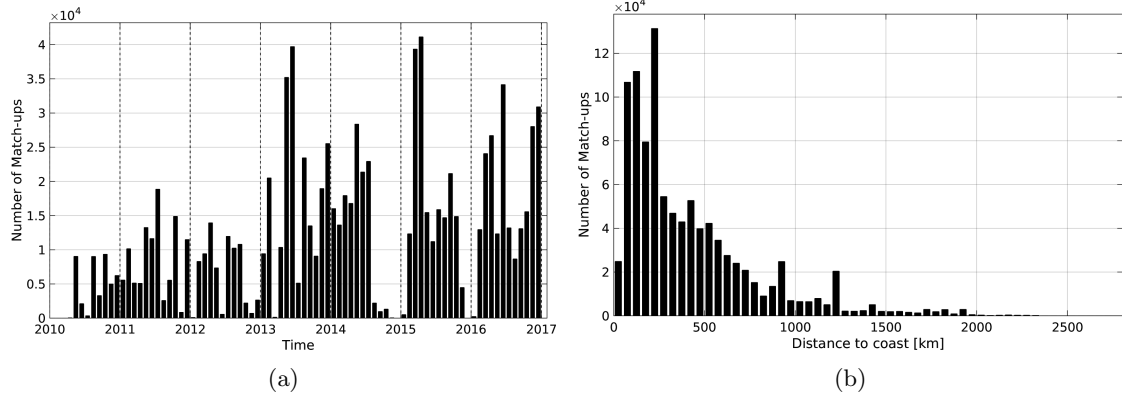
Figure 1: Number of match-ups between TSG-GOSUD-Research-vessel and SMOS-L3-CATDS-IFREMER-CECOS-V2-MONTHLY-0.25DEG SSS as a function of time (a) and as function of the distance to coast (b) over the Mid-Low Latitudes 45N-45S Pi-MEP region and for the full satellite product period.
