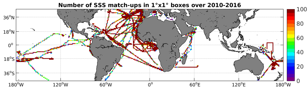
Figure 4: Number of SSS match-ups between TSG-GOSUD-Research-vessel SSS and the SMOS-L3-CATDS-IFREMER-CECOS-V2-MONTHLY-0.25DEG SSS product for the Mid-Low Latitudes 45N-45S Pi-MEP region over 1^\circ \times 1^\circ boxes and for the full satellite product period.
