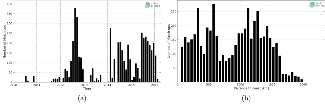
Figure 1: Number of match-ups between Sea mammals and SMOS SSS L3 v2 - Monthly - 0.25 Deg (CATDS-CECOS-IFREMER) SSS as a function of time (a) and as function of the distance to coast (b) over the Mid-Low Latitudes 45N-45S Pi-MEP region and for the full satellite product period.
