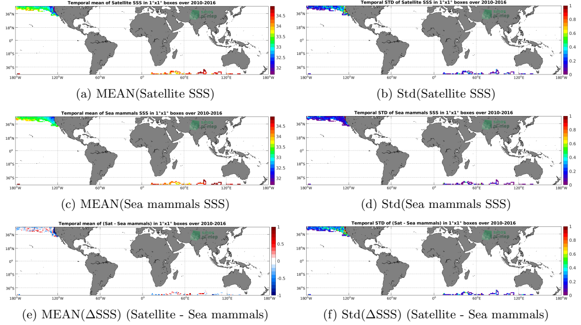
Figure 6: Temporal mean (left) and Std (right) of SSS from SMOS SSS L3 v2 - Monthly - 0.25 Deg (CATDS-CECOS-IFREMER) (top), Sea mammals (middle), and of \Delta SSS (Satellite - Sea mammals). Only match-up pairs are used to generate these maps.
