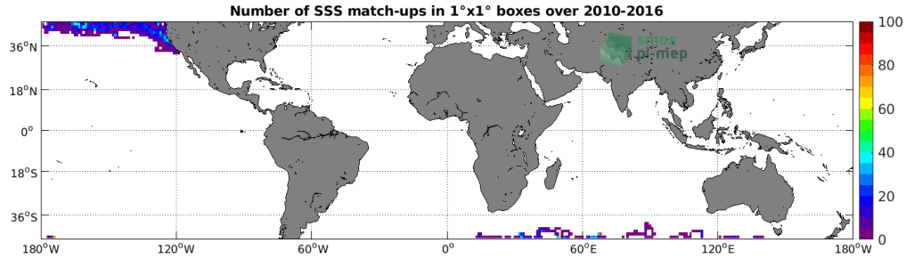
Figure 4: Number of SSS match-ups between Sea mammals SSS and the SMOS SSS L3 v2 - Monthly - 0.25 Deg (CATDS-CECOS-IFREMER) SSS product for the Mid-Low Latitudes 45N-45S Pi-MEP region over 1^\circ \times 1^\circ boxes and for the full satellite product period.
