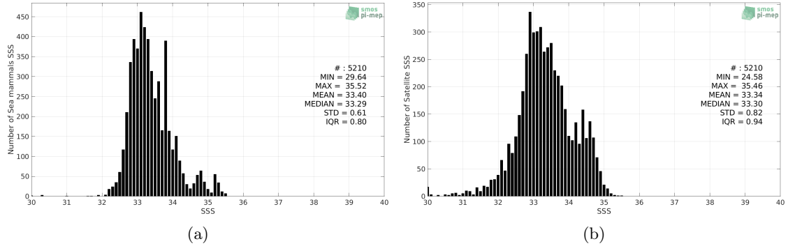
Figure 2: Histograms of SSS from Sea mammals (a) and SMOS SSS L3 v2 - Monthly - 0.25 Deg (CATDS-CECOS-IFREMER) (b) considering all match-up pairs per bins of 0.1 over the Mid-Low Latitudes 45N-45S Pi-MEP region and for the full satellite product period.
