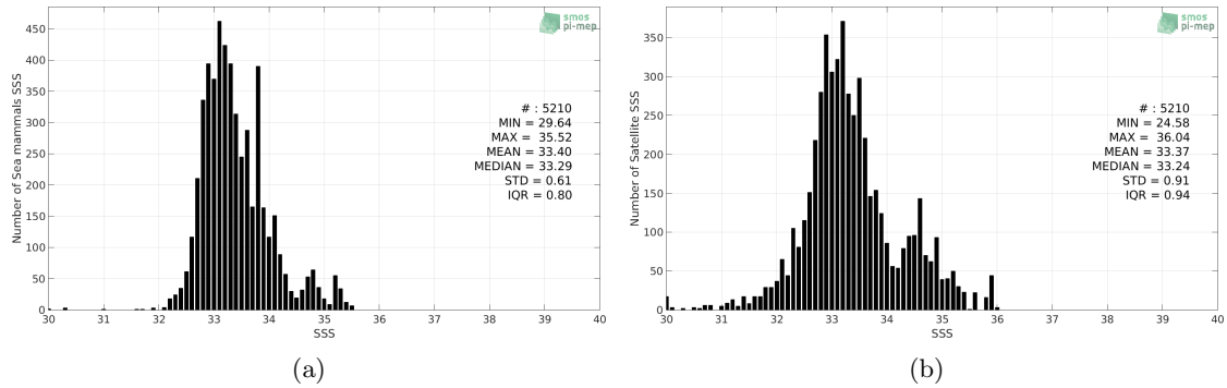
Figure 2: Histograms of SSS from Sea mammals (a) and SMOS L3 v2 - Monthly - 0.25 Deg (CATDS-CECOS-IFREMER) (b) considering all match-up pairs per bins of 0.1 over the Mid-Low Latitudes 45N-45S Pi-MEP region and for the full satellite product period.
