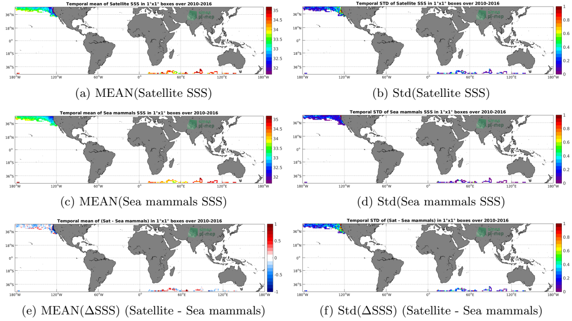
Figure 6: Temporal mean (left) and Std (right) of SSS from SMOS L3 v2 - Monthly - 0.25 Deg (CATDS-CECOS-IFREMER) (top), Sea mammals (middle), and of \Delta SSS (Satellite - Sea mammals). Only match-up pairs are used to generate these maps.
