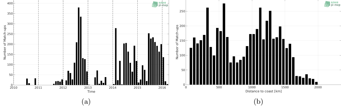
Figure 1: Number of match-ups between Sea mammals and SMOS L3 v2 - Monthly - 0.25 Deg (CATDS-CECOS-IFREMER) SSS as a function of time (a) and as function of the distance to coast (b) over the Mid-Low Latitudes 45N-45S Pi-MEP region and for the full satellite product period.
