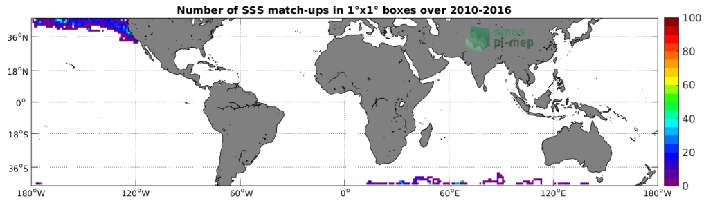
Figure 4: Number of SSS match-ups between Sea mammals SSS and the SMOS L3 v2 - Monthly - 0.25 Deg (CATDS-CECOS-IFREMER) SSS product for the Mid-Low Latitudes 45N-45S Pi-MEP region over 1°x1° boxes and for the full satellite product period.
