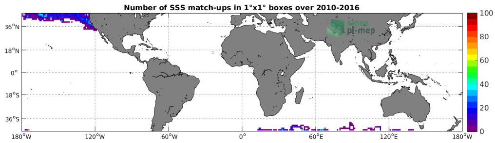
Figure 4: Number of SSS match-ups between Sea mammals SSS and the SMOS-L3-CATDS-IFREMER-CECOS-V2-MONTHLY-0.25DEG SSS product for the Mid-Low Latitudes 45N-45S Pi-MEP region over 1^\circ \times 1^\circ boxes and for the full satellite product period.
