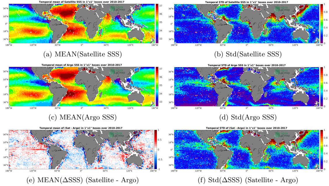
Figure 6: Temporal mean (left) and Std (right) of SSS from SMOS SSS L3 v2 - Monthly - 0.25 Deg (CATDS-CECOS-IFREMER) (top), Argo (middle), and of \Delta SSS (Satellite - Argo). Only match-up pairs are used to generate these maps.
