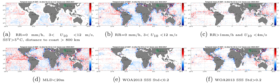
Figure 12: Temporal mean gridded over spatial boxes of size 1^\circ \times 1^\circ of \Delta SSS (SMOS SSS L3 v2 - Monthly - 0.25 Deg (CATDS-CECOS-IFREMER) - Argo) for 6 different subdatasets corresponding to: RR=0 mm/h, 3 < U_{10} < 12 m/s, SST > 5^\circ C , distance to coast > 800 km (a), RR=0 mm/h, 3 < U_{10} < 12 m/s (b), RR > 1 mm/h and U_{10} < 4 m/s (c), MLD < 20 m (d), WOA2013 SSS Std < 0.2 (e), WOA2013 SSS Std > 0.2 (f).
