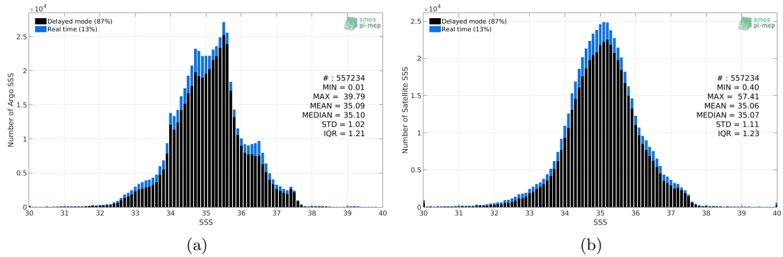
Figure 2: Histograms of SSS from Argo (a) and SMOS SSS L3 v2 - Monthly - 0.25 Deg (CATDS-CECOS-IFREMER) (b) considering all match-up pairs per bins of 0.1 over the Mid-Low Latitudes 45N-45S Pi-MEP region and for the full satellite product period.
