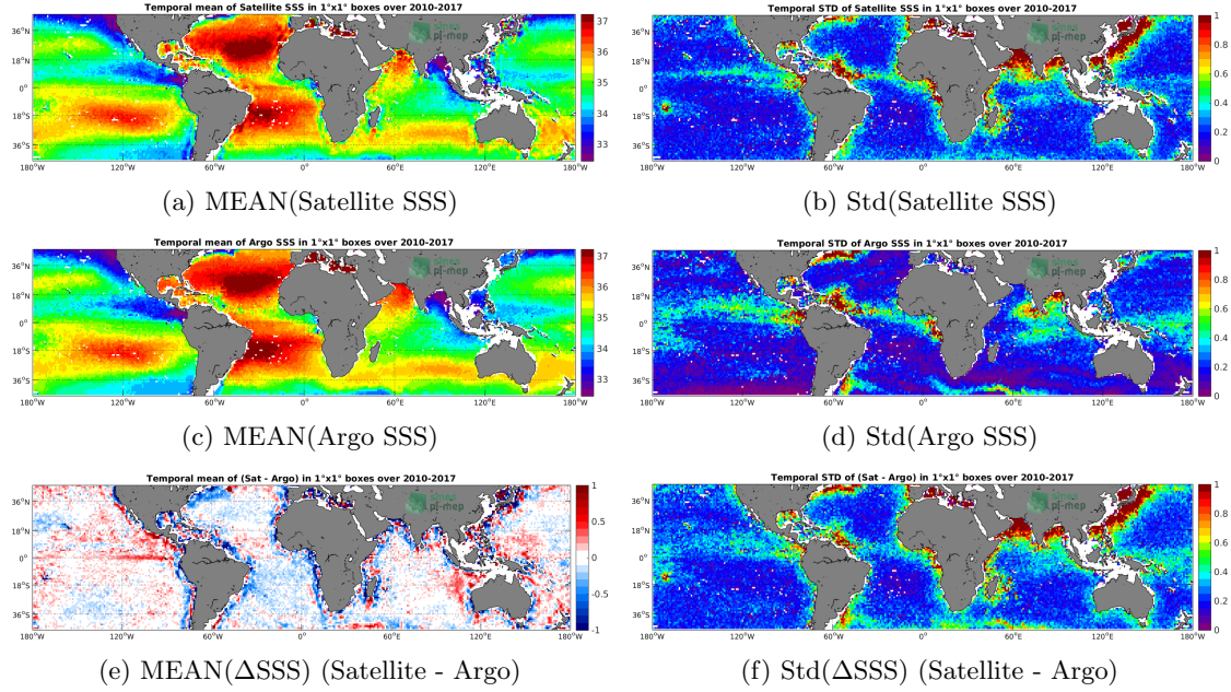
Figure 6: Temporal mean (left) and Std (right) of SSS from SMOS SSS L3 v2 - Monthly - 0.25 Deg (CATDS-CECOS-IFREMER) (top), Argo (middle), and of \Delta SSS (Satellite - Argo). Only match-up pairs are used to generate these maps.
