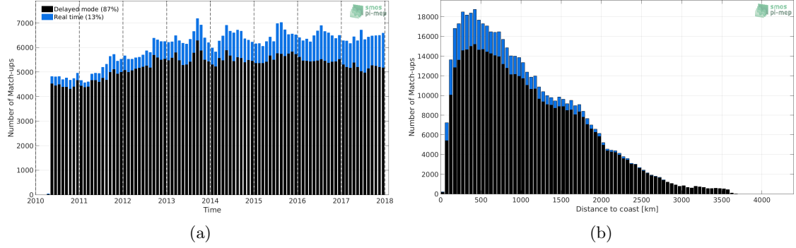
Figure 1: Number of match-ups between Argo and SMOS SSS L3 v2 - Monthly - 0.25 Deg (CATDS-CECOS-IFREMER) SSS as a function of time (a) and as function of the distance to coast (b) over the Mid-Low Latitudes 45N-45S Pi-MEP region and for the full satellite product period.
