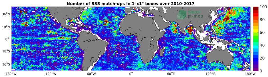
Figure 4: Number of SSS match-ups between Argo SSS and the SMOS SSS L3 v2 - Monthly - 0.25 Deg (CATDS-CECOS-IFREMER) SSS product for the Mid-Low Latitudes 45N-45S Pi-MEP region over 1°x1° boxes and for the full satellite product period.
