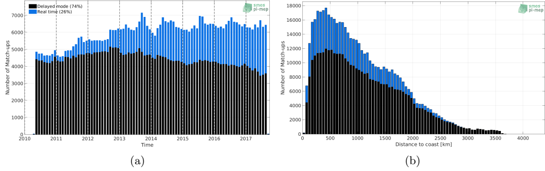
Figure 1: Number of match-ups between Argo and SMOS-L3-CATDS-IFREMER-CECOS-V2-MONTHLY-0.25DEG SSS as a function of time (a) and as function of the distance to coast (b) over the Mid-Low Latitudes 45N-45S Pi-MEP region and for the full satellite product period.
