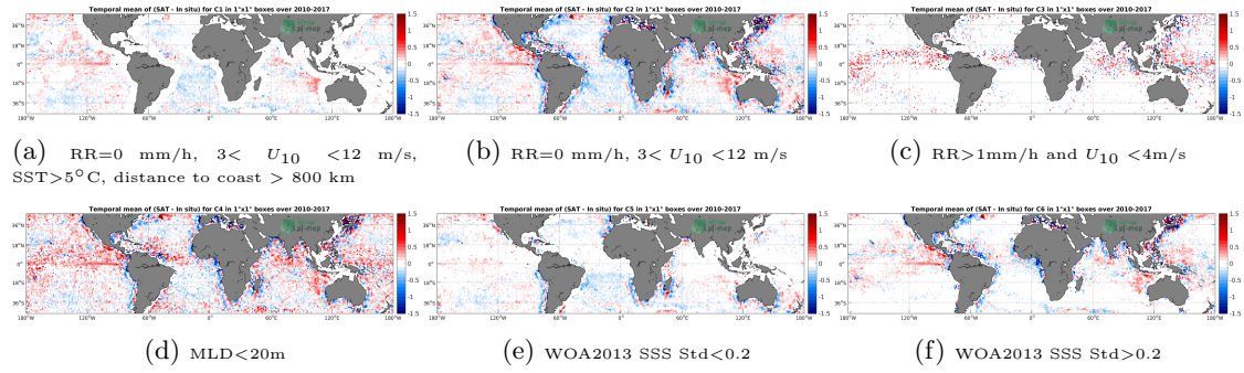
Figure 12: Temporal mean gridded over spatial boxes of size 1^\circ \times 1^\circ of \Delta SSS (SMOS-L3-CATDS-IFREMER-CECOS-V2-MONTHLY-0.25DEG - Argo) for 6 different subdatasets corresponding to:RR=0 mm/h, 3 < U_{10} < 12 m/s, SST >5^\circ\text{C} , distance to coast > 800 km (a), RR=0 mm/h, 3 < U_{10} < 12 m/s (b), RR >1 mm/h and U_{10} < 4 m/s (c),MLD <20 m (d),WOA2013 SSS Std <0.2 (e),WOA2013 SSS Std >0.2 (f).
