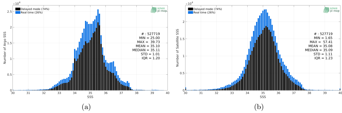
Figure 2: Histograms of SSS from Argo (a) and SMOS-L3-CATDS-IFREMER-CECOS-V2-MONTHLY-0.25DEG (b) considering all match-up pairs per bins of 0.1 over the Mid-Low Latitudes 45N-45S Pi-MEP region and for the full satellite product period.
