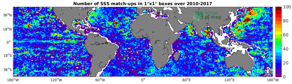
Figure 4: Number of SSS match-ups between Argo SSS and the SMOS-L3-CATDS-IFREMER-CECOS-V2-MONTHLY-0.25DEG SSS product for the Mid-Low Latitudes 45N-45S Pi-MEP region over 1°x1° boxes and for the full satellite product period.
