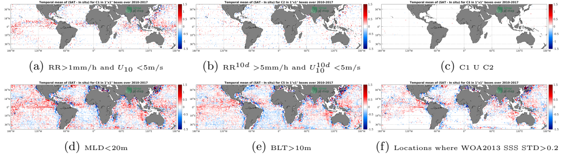
Figure 12: Temporal mean gridded over spatial boxes of size 1^\circ \times 1^\circ of \Delta SSS (SMOS-L3-CATDS-IFREMER-CECOS-V2-MONTHLY-0.25DEG - Argo) for 6 different subdatasets corresponding to: RR>1\text{mm/h} and U_{10}<5\text{m/s} (a), RR^{10d}>5\text{mm/h} and U_{10}^{10d}<5\text{m/s} (b), C1 U C2 (c), MLD<20\text{m} (d), BLT>10\text{m} (e), Locations where WOA2013 SSS STD>0.2 (f).
