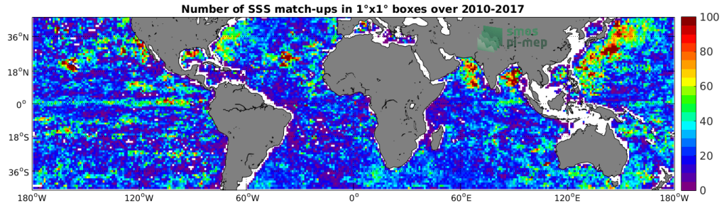
Figure 4: Number of SSS match-ups between Argo SSS and the SMOS-L3-CATDS-IFREMER-CECOS-V2-MONTHLY-0.25DEG SSS product for the Mid-Low Latitudes 45N-45S Pi-MEP region over 1^\circ \times 1^\circ boxes and for the full satellite product period.
