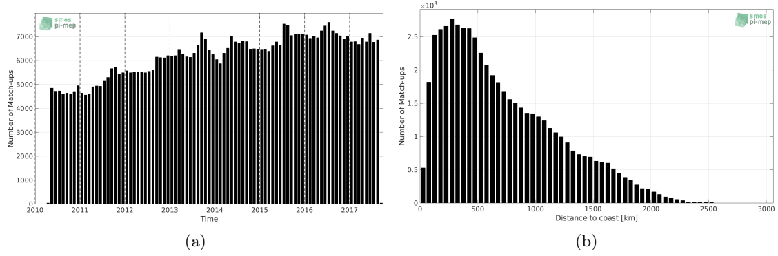
Figure 1: Number of match-ups between Argo and SMOS-L3-CATDS-IFREMER-CECOS-V2-MONTHLY-0.25DEG SSS as a function of time (a) and as function of the distance to coast (b) over the Mid-Low Latitudes 45N-45S Pi-MEP region and for the full satellite product period.
