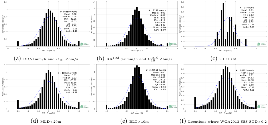
Figure 13: Normalized histogram of \Delta SSS (SMOS-L3-CATDS-IFREMER-CECOS-V2-MONTHLY-0.25DEG - Argo) for 6 different subdatasets corresponding to: RR>1\text{mm/h} and U_{10}<5\text{m/s} (a), RR^{10d}>5\text{mm/h} and U_{10}^{10d}<5\text{m/s} (b), C1 U C2 (c), MLD<20\text{m} (d), BLT>10\text{m} (e), Locations where WOA2013 SSS STD>0.2 (f).
