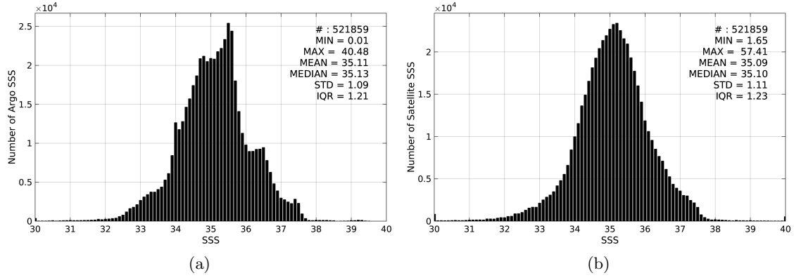
Figure 2: Histograms of SSS from Argos (a) and SMOS-L3-CATDS-IFREMER-CECOS-V2-MONTHLY-0.25DEG (b) considering all match-up pairs per bins of 0.1 over the Mid-Low Latitudes 45N-45S Pi-MEP region and for the full satellite product period.
