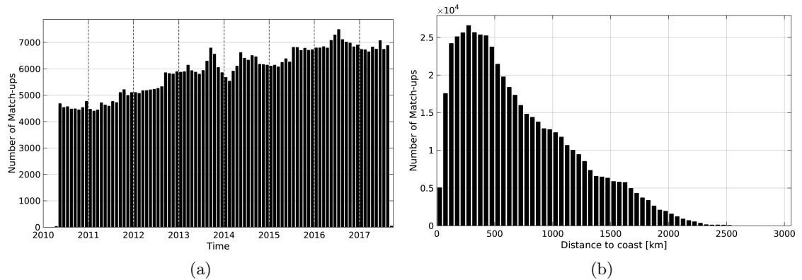
Figure 1: Number of match-ups between Argo and SMOS-L3-CATDS-IFREMER-CECOS-V2-MONTHLY-0.25DEG SSS as a function of time (a) and as function of the distance to coast (b) over the Mid-Low Latitudes 45N-45S Pi-MEP region and for the full satellite product period.
