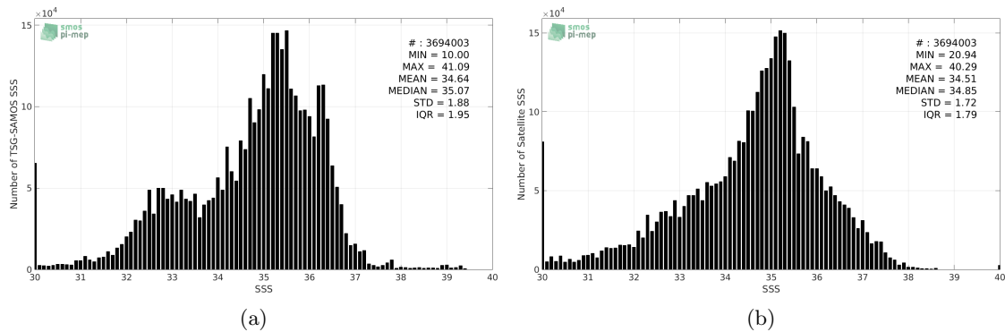
Figure 2: Histograms of SSS from TSG-SAMOS (a) and SMOS-L3-CATDS-CECOS-IFREMER-V2-1DAY-0.5DEG (b) considering all match-up pairs per bins of 0.1 over the Mid-Low Latitudes 45N-45S Pi-MEP region and for the full satellite product period.
