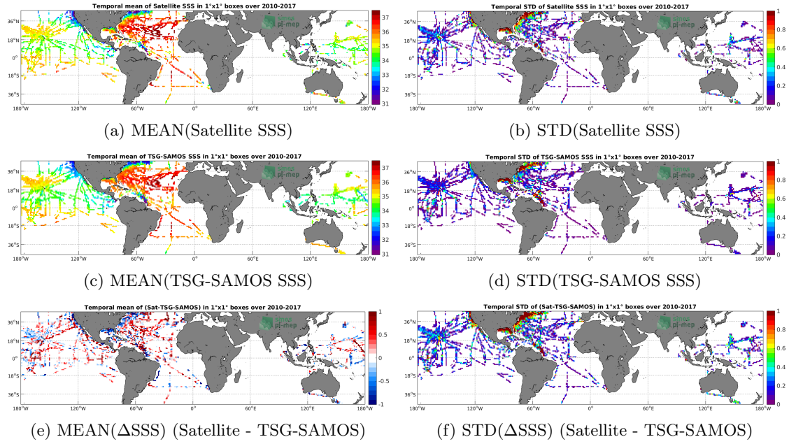
Figure 6: Temporal mean (left) and STD (right) of SSS from SMOS-L3-CATDS-CECOS-IFREMER-V2-1DAY-0.5DEG (top), TSG-SAMOS (middle), and of \Delta SSS (Satellite - TSG-SAMOS). Only match-up pairs are used to generate these maps.
