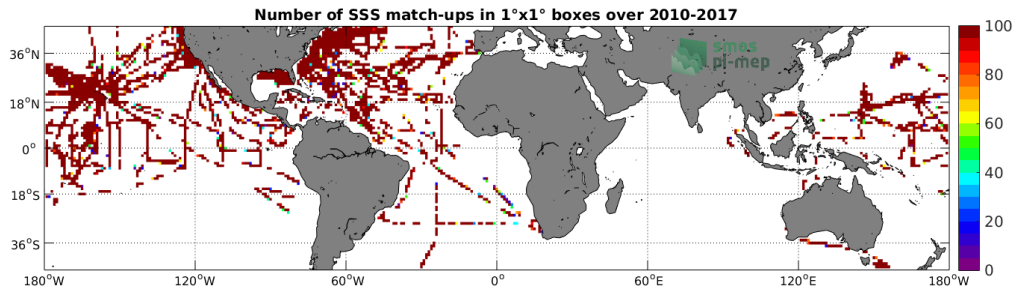
Figure 4: Number of SSS match-ups between TSG-SAMOS SSS and the SMOS-L3-CATDS-CECOS-IFREMER-V2-1DAY-0.5DEG SSS product for the Mid-Low Latitudes 45N-45S Pi-MEP region over 1^\circ \times 1^\circ boxes and for the full satellite product period.
