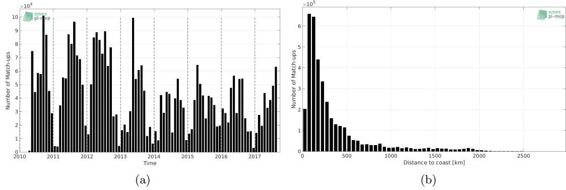
Figure 1: Number of match-ups between TSG-SAMOS and SMOS-L3-CATDS-CECOS-IFREMER-V2-1DAY-0.5DEG SSS as a function of time (a) and as function of the distance to coast (b) over the Mid-Low Latitudes 45N-45S Pi-MEP region and for the full satellite product period.
