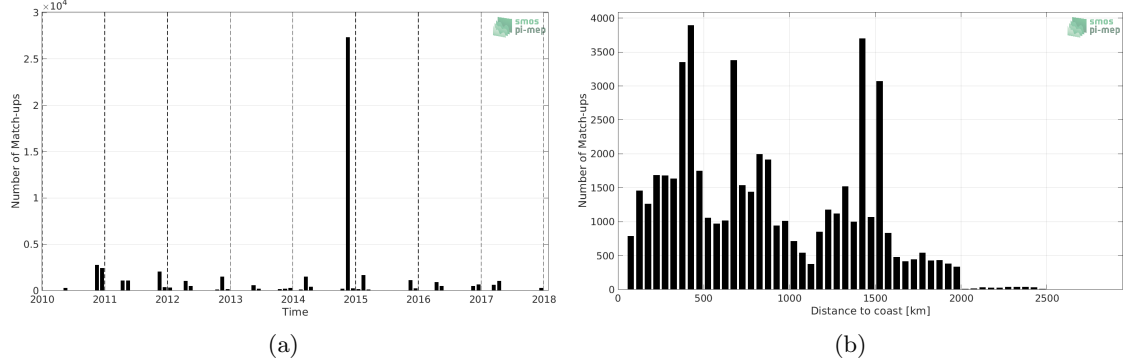
Figure 1: Number of match-ups between TSG (Polarstern) and SMOS SSS L3 v2 - Daily - 0.5 Deg (CATDS-CECOS-IFREMER) SSS as a function of time (a) and as function of the distance to coast (b) over the Mid-Low Latitudes 45N-45S Pi-MEP region and for the full satellite product period.
