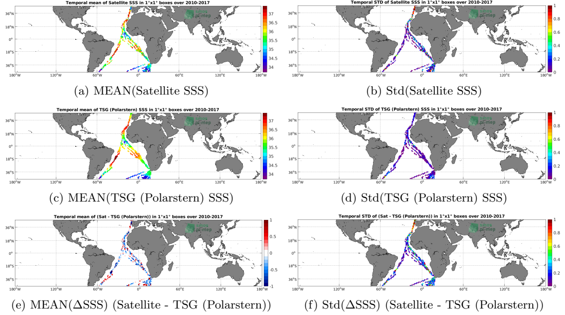
Figure 6: Temporal mean (left) and Std (right) of SSS from SMOS SSS L3 v2 - Daily - 0.5 Deg (CATDS-CECOS-IFREMER) (top), TSG (Polarstern) (middle), and of \Delta SSS (Satellite - TSG (Polarstern)). Only match-up pairs are used to generate these maps.
