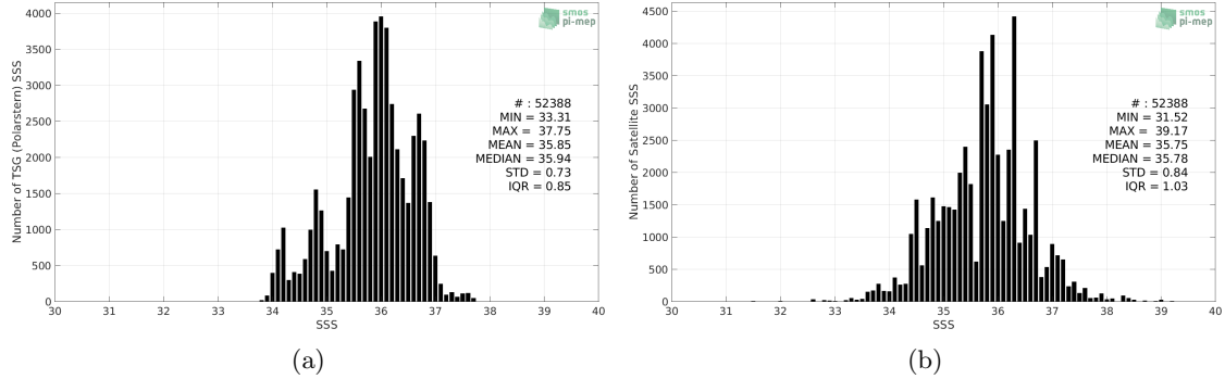
Figure 2: Histograms of SSS from TSG (Polarstern) (a) and SMOS SSS L3 v2 - Daily - 0.5 Deg (CATDS-CECOS-IFREMER) (b) considering all match-up pairs per bins of 0.1 over the Mid-Low Latitudes 45N-45S Pi-MEP region and for the full satellite product period.
