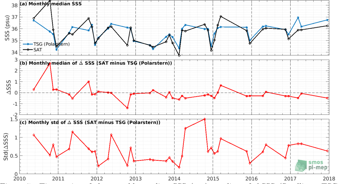
Figure 7: Time series of the monthly median SSS (top), median of \Delta\text{SSS} (Satellite - TSG (Polarstern)) and Std of \Delta\text{SSS} (Satellite - TSG (Polarstern)) over the Mid-Low Latitudes 45N-45S Pi-MEP region considering all match-ups collected by the Pi-MEP.
