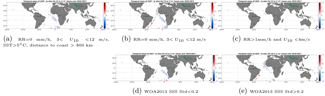
Figure 12: Temporal mean gridded over spatial boxes of size 1^\circ \times 1^\circ of \Delta SSS (SMOS SSS L3 v2 - Daily - 0.5 Deg (CATDS-CECOS-IFREMER) - TSG (Polarstern)) for 5 different subdatasets corresponding to: RR=0 mm/h, 3 < U_{10} < 12 m/s, SST > 5^\circ C , distance to coast > 800 km (a), RR=0 mm/h, 3 < U_{10} < 12 m/s (b), RR > 1 mm/h and U_{10} < 4 m/s (c), WOA2013 SSS Std < 0.2 (d), WOA2013 SSS Std > 0.2 (e).
