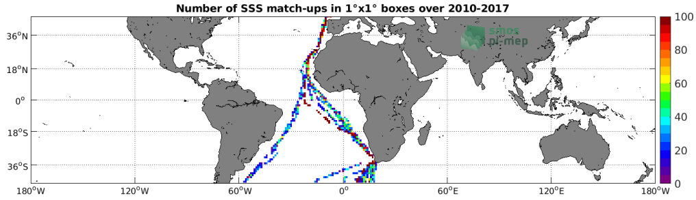
Figure 4: Number of SSS match-ups between TSG (Polarstern) SSS and the SMOS SSS L3 v2 - Daily - 0.5 Deg (CATDS-CECOS-IFREMER) SSS product for the Mid-Low Latitudes 45N-45S Pi-MEP region over 1^\circ \times 1^\circ boxes and for the full satellite product period.
