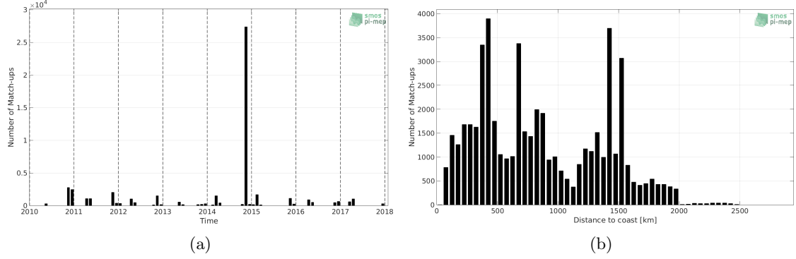
Figure 1: Number of match-ups between TSG (Polarstern) and SMOS SSS L3 v2 - Daily - 0.5 Deg (CATDS-CECOS-IFREMER) SSS as a function of time (a) and as function of the distance to coast (b) over the Mid-Low Latitudes 45N-45S Pi-MEP region and for the full satellite product period.
