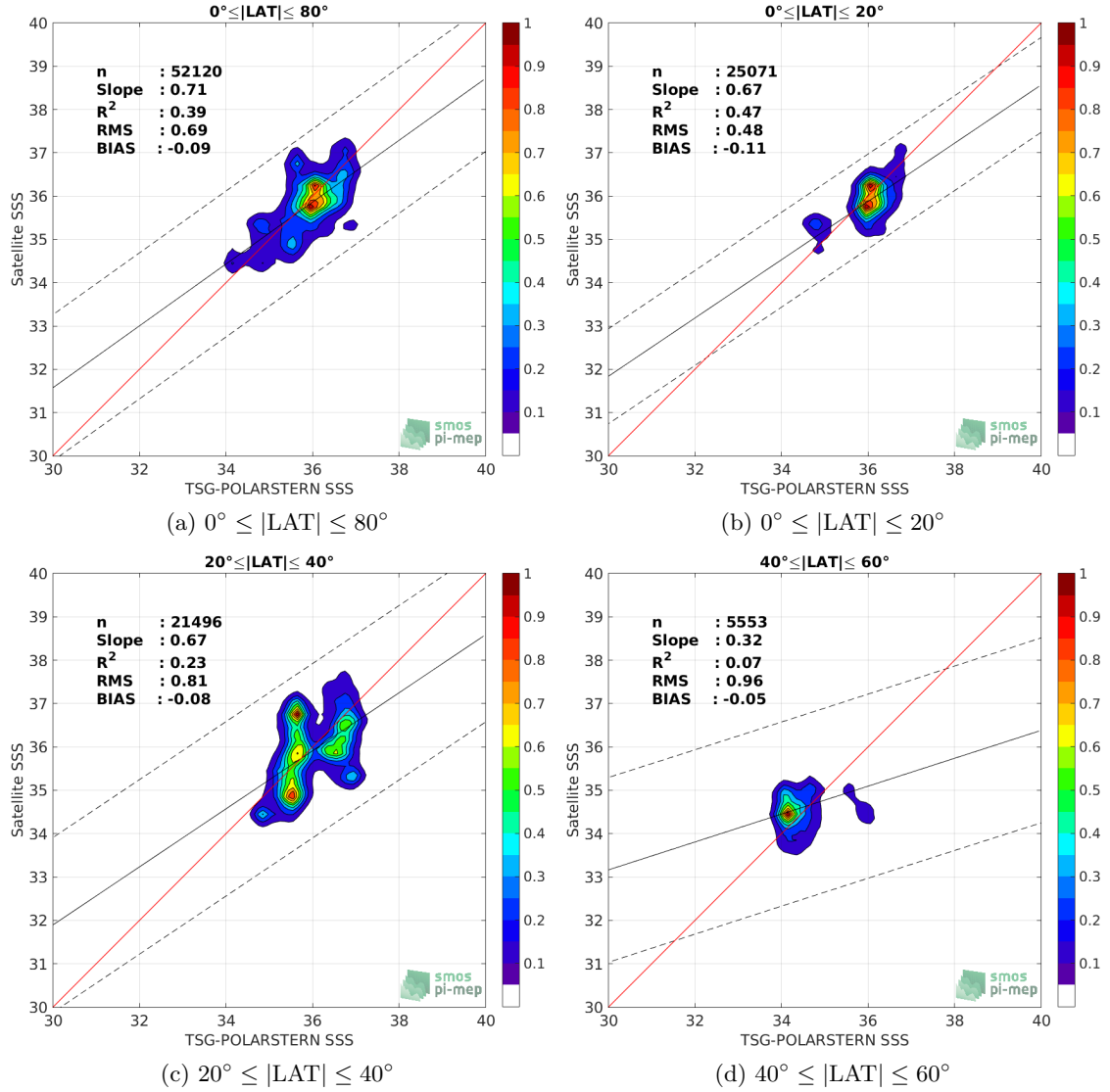
Figure 9: Contour maps of the concentration of SMOS L3 v2 - Daily - 0.5 Deg (CATDS-CECOS-IFREMER) SSS (y-axis) versus TSG-POLARSTERN SSS (x-axis) at match-up pairs for different latitude bands. For each plot, the red line shows x=y . The black thin and dashed lines indicate a linear fit through the data cloud and the \pm 95\% confidence levels, respectively. The number match-up pairs n , the slope and R^2 coefficient of the linear fit, the root mean square (RMS) and the mean bias between satellite and in situ data are indicated for each latitude band in each plots.
