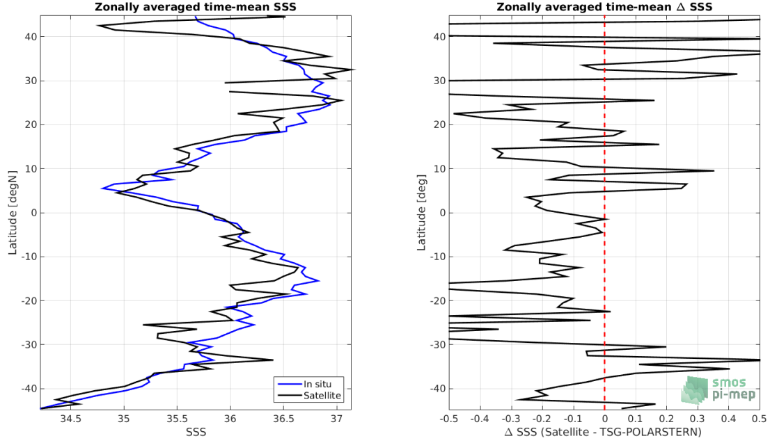
Figure 8: Left panel: Zonal mean SSS from SMOS L3 v2 - Daily - 0.5 Deg (CATDS-CECOS-IFREMER) satellite product (black) and from TSG-POLARSTERN (blue). Right panel: Zonal mean of \Delta SSS (Satellite - TSG-POLARSTERN) for all the collected Pi-MEP match-up pairs estimated over the full satellite product period.
