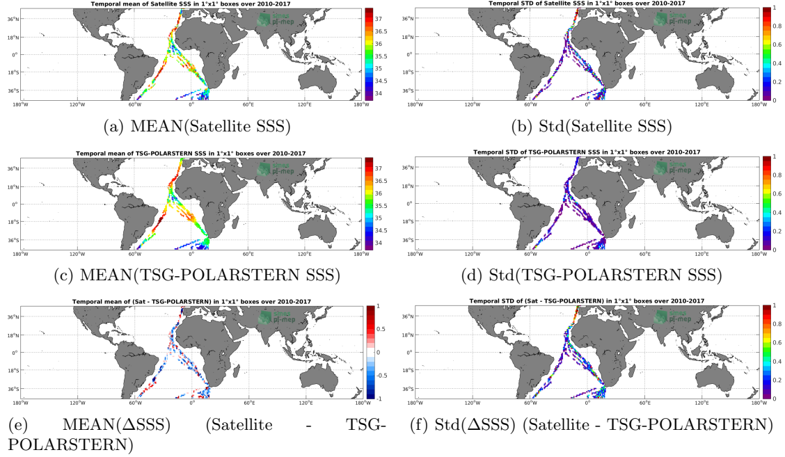
Figure 6: Temporal mean (left) and Std (right) of SSS from SMOS L3 v2 - Daily - 0.5 Deg (CATDS-CECOS-IFREMER) (top), TSG-POLARSTERN (middle), and of \Delta SSS (Satellite - TSG-POLARSTERN). Only match-up pairs are used to generate these maps.
