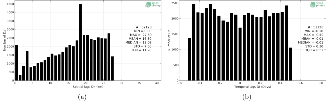
Figure 5: Histograms of the spatial (a) and temporal (b) lags between the time of the TSG-POLARSTERN measurements and the date of the corresponding SMOS L3 v2 - Daily - 0.5 Deg (CATDS-CECOS-IFREMER) SSS product.
