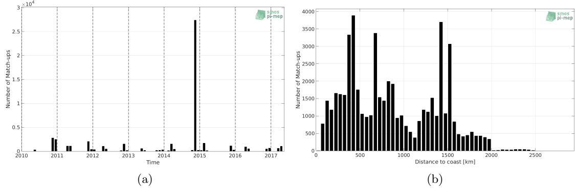
Figure 1: Number of match-ups between TSG-POLARSTERN and SMOS L3 v2 - Daily - 0.5 Deg (CATDS-CECOS-IFREMER) SSS as a function of time (a) and as function of the distance to coast (b) over the Mid-Low Latitudes 45N-45S Pi-MEP region and for the full satellite product period.
