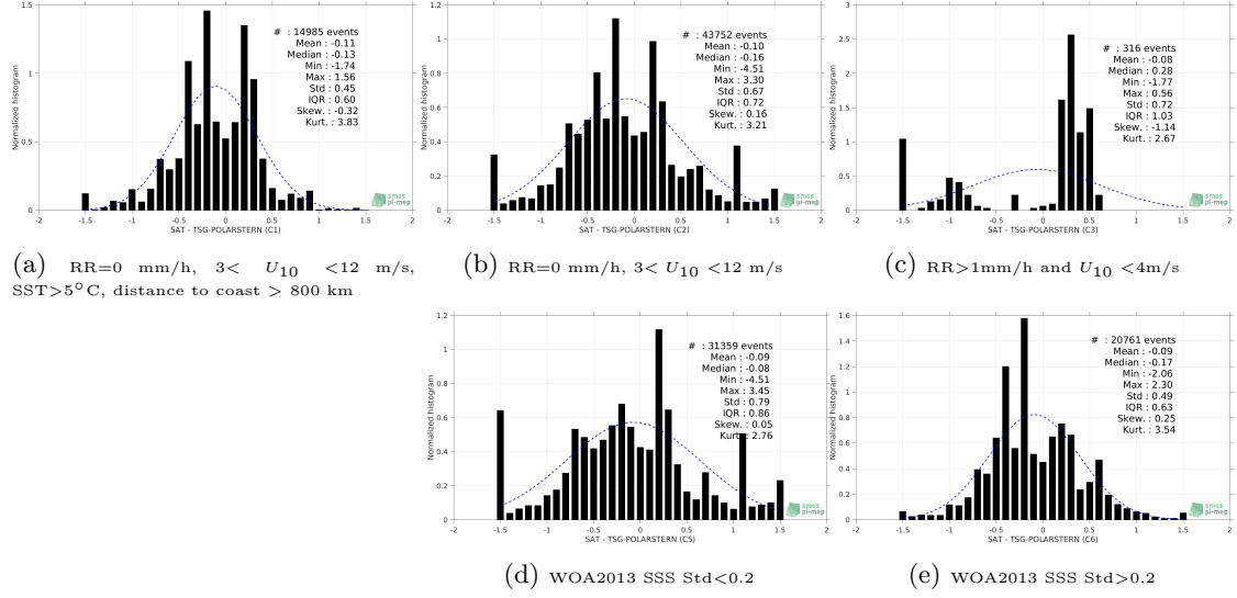
Figure 13: Normalized histogram of \Delta SSS (SMOS L3 v2 - Daily - 0.5 Deg (CATDS-CECOS-IFREMER) - TSG-POLARSTERN) for 5 different subdatasets corresponding to: RR=0 mm/h, 3 < U_{10} < 12 m/s, SST>5°C, distance to coast > 800 km (a), RR=0 mm/h, 3 < U_{10} < 12 m/s (b), RR>1mm/h and U_{10} < 4 m/s (c), WOA2013 SSS Std<0.2 (d), WOA2013 SSS Std>0.2 (e).
