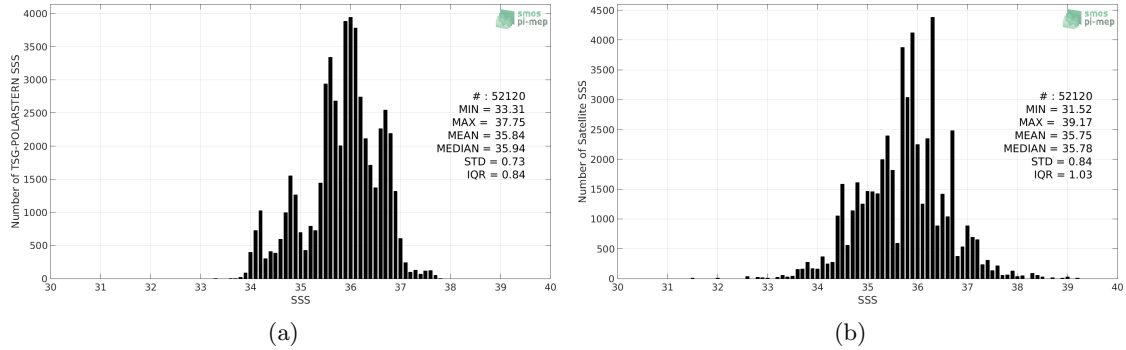
Figure 2: Histograms of SSS from TSG-POLARSTERN (a) and SMOS L3 v2 - Daily - 0.5 Deg (CATDS-CECOS-IFREMER) (b) considering all match-up pairs per bins of 0.1 over the Mid-Low Latitudes 45N-45S Pi-MEP region and for the full satellite product period.
