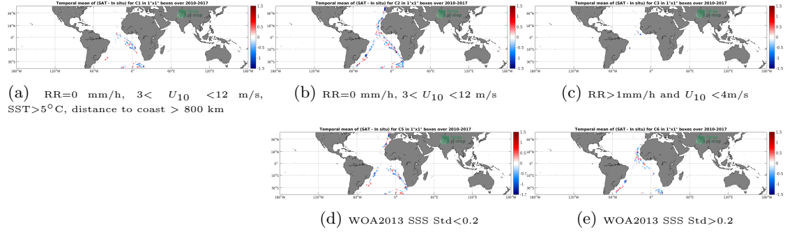
Figure 12: Temporal mean gridded over spatial boxes of size 1^\circ \times 1^\circ of \Delta SSS (SMOS L3 v2 - Daily - 0.5 Deg (CATDS-CECOS-IFREMER) - TSG-POLARSTERN) for 5 different subdatasets corresponding to: RR=0 mm/h, 3 < U_{10} < 12 m/s, SST > 5^\circ C , distance to coast > 800 km (a), RR=0 mm/h, 3 < U_{10} < 12 m/s (b), RR > 1 mm/h and U_{10} < 4 m/s (c), WOA2013 SSS Std < 0.2 (d), WOA2013 SSS Std > 0.2 (e).
