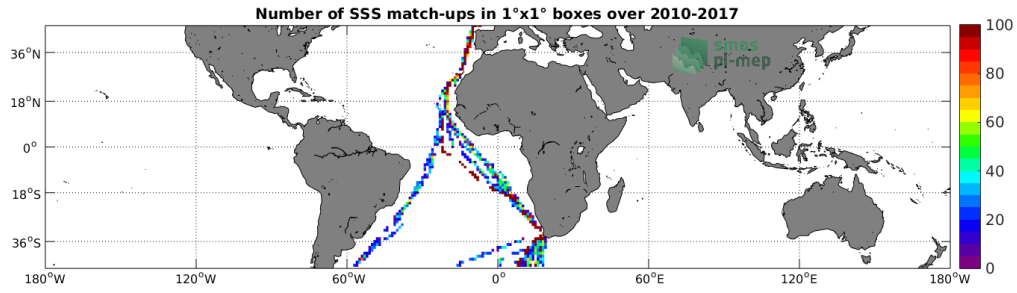
Figure 4: Number of SSS match-ups between TSG-POLARSTERN SSS and the SMOS L3 v2 - Daily - 0.5 Deg (CATDS-CECOS-IFREMER) SSS product for the Mid-Low Latitudes 45N-45S Pi-MEP region over 1^\circ \times 1^\circ boxes and for the full satellite product period.
