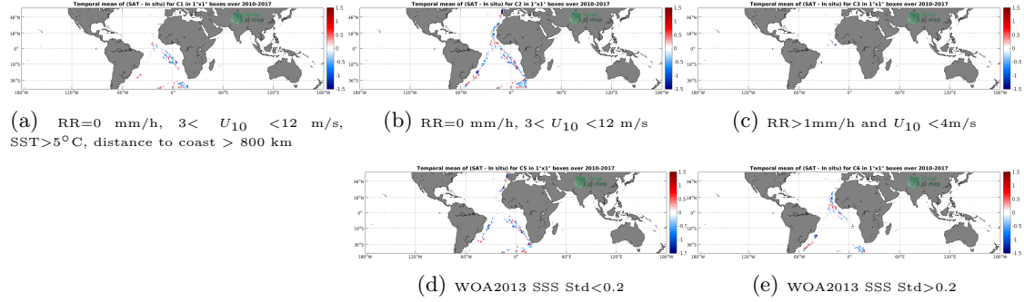
Figure 12: Temporal mean gridded over spatial boxes of size 1^\circ \times 1^\circ of \Delta SSS (SMOS-L3-CATDS-CECOS-IFREMER-V2-1DAY-0.5DEG - TSG-POLARSTERN) for 5 different subdatasets corresponding to: RR=0 mm/h, 3 < U_{10} < 12 m/s, SST > 5^\circ C , distance to coast > 800 km (a), RR=0 mm/h, 3 < U_{10} < 12 m/s (b), RR > 1 mm/h and U_{10} < 4 m/s (c), WOA2013 SSS Std < 0.2 (d), WOA2013 SSS Std > 0.2 (e).
