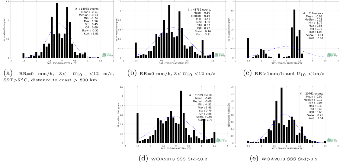
Figure 13: Normalized histogram of \Delta SSS (SMOS-L3-CATDS-CECOS-IFREMER-V2-1DAY-0.5DEG - TSG-POLARSTERN) for 5 different subdatasets corresponding to: RR=0 mm/h, 3 < U_{10} < 12 m/s, SST>5°C, distance to coast > 800 km (a), RR=0 mm/h, 3 < U_{10} < 12 m/s (b), RR>1mm/h and U_{10} < 4 m/s (c), WOA2013 SSS Std<0.2 (d), WOA2013 SSS Std>0.2 (e).
