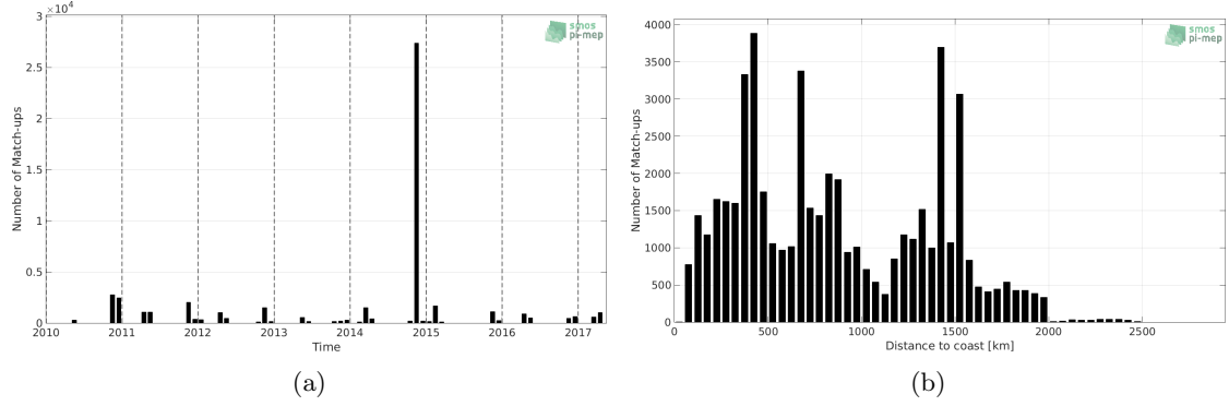
Figure 1: Number of match-ups between TSG-POLARSTERN and SMOS-L3-CATDS-CECOS-IFREMER-V2-1DAY-0.5DEG SSS as a function of time (a) and as function of the distance to coast (b) over the Mid-Low Latitudes 45N-45S Pi-MEP region and for the full satellite product period.
