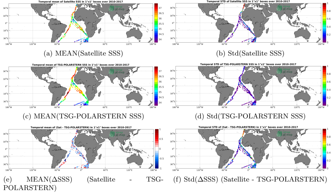
Figure 6: Temporal mean (left) and Std (right) of SSS from SMOS-L3-CATDS-CECOS-IFREMER-V2-1DAY-0.5DEG (top), TSG-POLARSTERN (middle), and of \Delta SSS (Satellite - TSG-POLARSTERN). Only match-up pairs are used to generate these maps.
