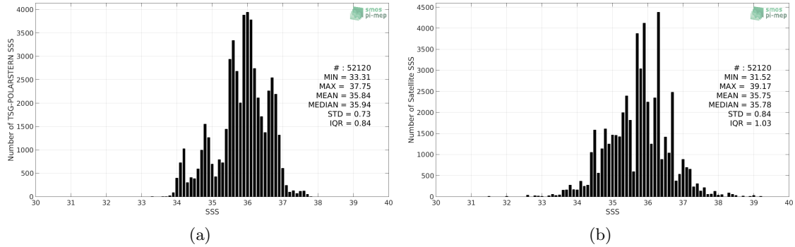
Figure 2: Histograms of SSS from TSG-POLARSTERN (a) and SMOS-L3-CATDS-CECOS-IFREMER-V2-1DAY-0.5DEG (b) considering all match-up pairs per bins of 0.1 over the Mid-Low Latitudes 45N-45S Pi-MEP region and for the full satellite product period.
