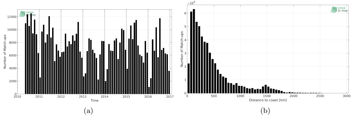
Figure 1: Number of match-ups between TSG-LEGOS-DM and SMOS-L3-CATDS-CECOS-IFREMER-V2-1DAY-0.5DEG SSS as a function of time (a) and as function of the distance to coast (b) over the Mid-Low Latitudes 45N-45S Pi-MEP region and for the full satellite product period.
