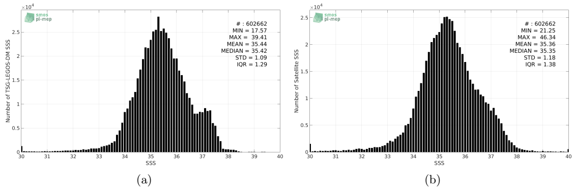
Figure 2: Histograms of SSS from TSG-LEGOS-DM (a) and SMOS-L3-CATDS-CECOS-IFREMER-V2-1DAY-0.5DEG (b) considering all match-up pairs per bins of 0.1 over the Mid-Low Latitudes 45N-45S Pi-MEP region and for the full satellite product period.
