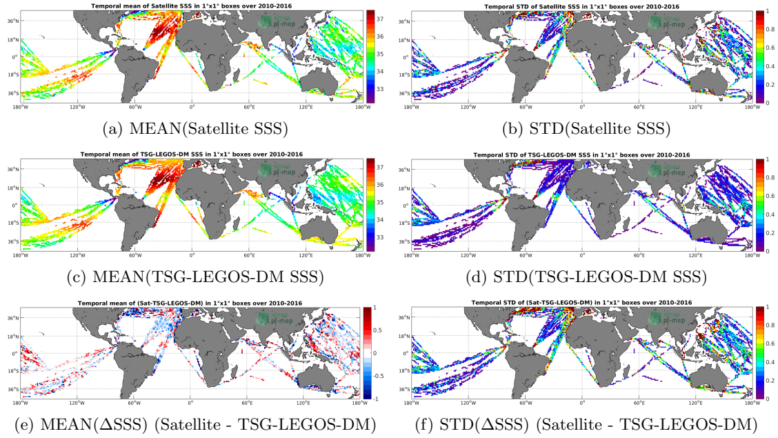
Figure 6: Temporal mean (left) and STD (right) of SSS from SMOS-L3-CATDS-CECOS-IFREMER-V2-1DAY-0.5DEG (top), TSG-LEGOS-DM (middle), and of \Delta SSS (Satellite - TSG-LEGOS-DM). Only match-up pairs are used to generate these maps.
