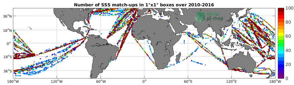
Figure 4: Number of SSS match-ups between TSG-LEGOS-DM SSS and the SMOS-L3-CATDS-CECOS-IFREMER-V2-1DAY-0.5DEG SSS product for the Mid-Low Latitudes 45N-45S Pi-MEP region over 1^\circ \times 1^\circ boxes and for the full satellite product period.
