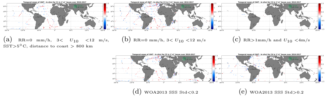
Figure 12: Temporal mean gridded over spatial boxes of size 1^\circ \times 1^\circ of \Delta SSS (SMOS SSS L3 v2 - Daily - 0.5 Deg (CATDS-CECOS-IFREMER) - TSG (GOSUD-Sailing-ship)) for 5 different subdatasets corresponding to: RR=0 mm/h, 3 < U_{10} < 12 m/s, SST > 5^\circ C , distance to coast > 800 km (a), RR=0 mm/h, 3 < U_{10} < 12 m/s (b), RR > 1 mm/h and U_{10} < 4 m/s (c), WOA2013 SSS Std < 0.2 (d), WOA2013 SSS Std > 0.2 (e).
