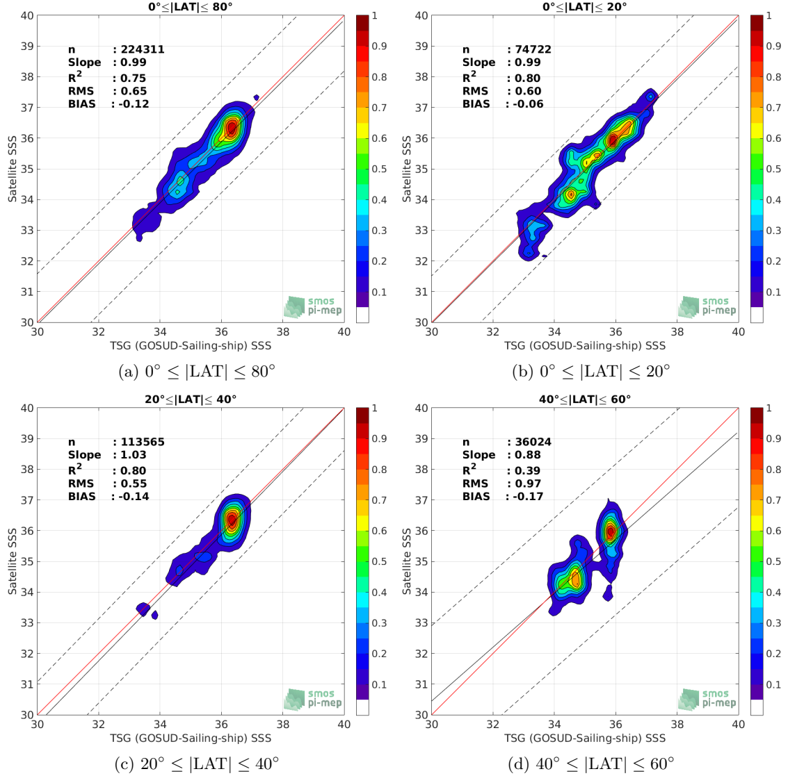
Figure 9: Contour maps of the concentration of SMOS SSS L3 v2 - Daily - 0.5 Deg (CATDS-CECOS-IFREMER) SSS (y-axis) versus TSG (GOSUD-Sailing-ship) SSS (x-axis) at match-up pairs for different latitude bands. For each plot, the red line shows x=y . The black thin and dashed lines indicate a linear fit through the data cloud and the \pm 95\% confidence levels, respectively. The number match-up pairs n , the slope and R^2 coefficient of the linear fit, the root mean square (RMS) and the mean bias between satellite and in situ data are indicated for each latitude band in each plots.
