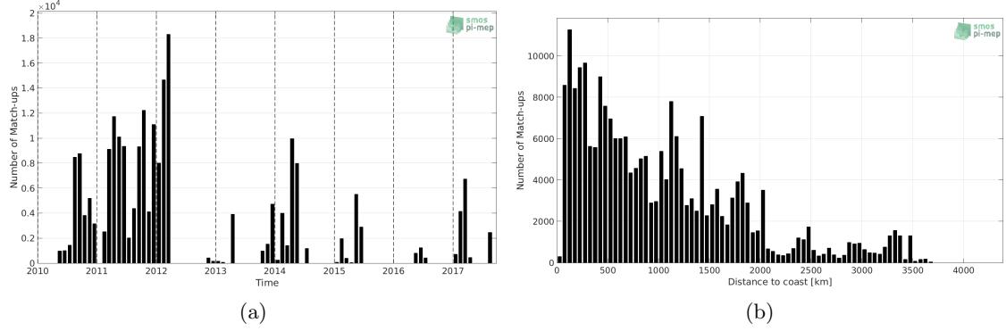
Figure 1: Number of match-ups between TSG (GOSUD-Sailing-ship) and SMOS SSS L3 v2 - Daily - 0.5 Deg (CATDS-CECOS-IFREMER) SSS as a function of time (a) and as function of the distance to coast (b) over the Mid-Low Latitudes 45N-45S Pi-MEP region and for the full satellite product period.
