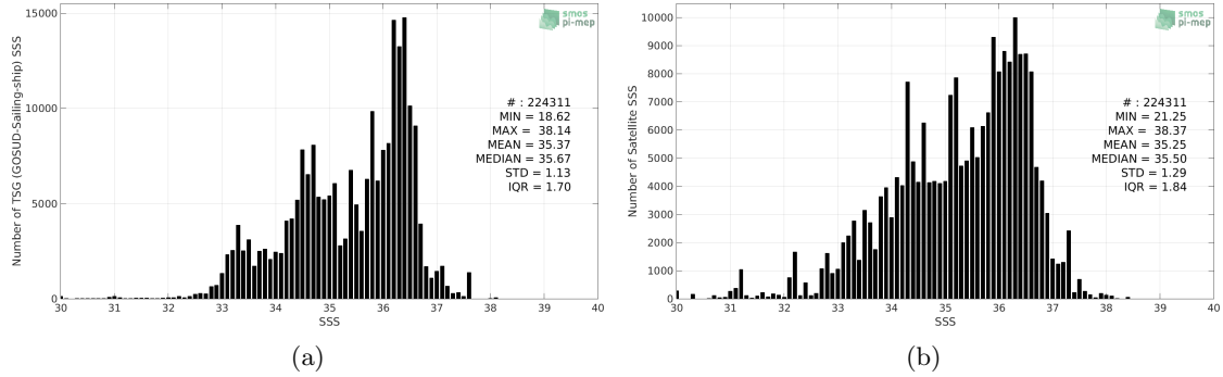
Figure 2: Histograms of SSS from TSG (GOSUD-Sailing-ship) (a) and SMOS SSS L3 v2 - Daily - 0.5 Deg (CATDS-CECOS-IFREMER) (b) considering all match-up pairs per bins of 0.1 over the Mid-Low Latitudes 45N-45S Pi-MEP region and for the full satellite product period.
