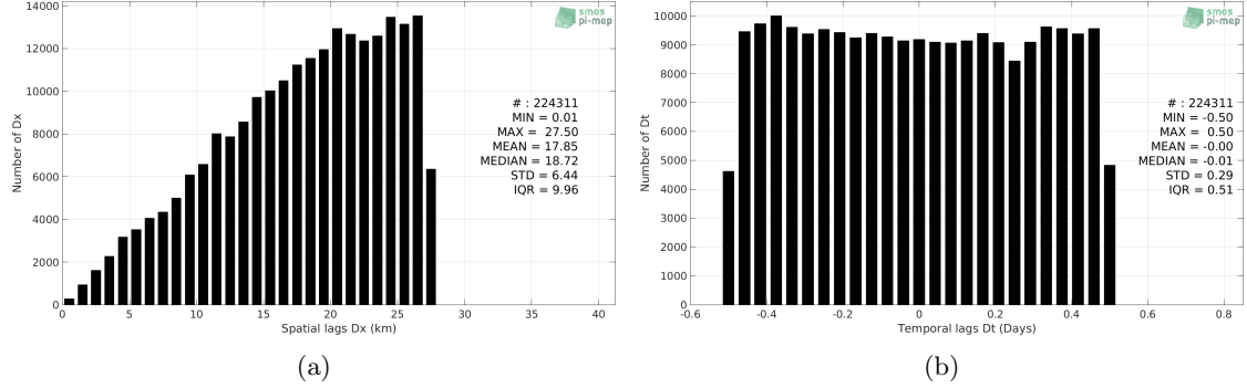
Figure 5: Histograms of the spatial (a) and temporal (b) lags between the time of the TSG (GOSUD-Sailing-ship) measurements and the date of the corresponding SMOS SSS L3 v2 - Daily - 0.5 Deg (CATDS-CECOS-IFREMER) SSS product.
