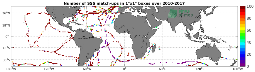
Figure 4: Number of SSS match-ups between TSG (GOSUD-Sailing-ship) SSS and the SMOS SSS L3 v2 - Daily - 0.5 Deg (CATDS-CECOS-IFREMER) SSS product for the Mid-Low Latitudes 45N-45S Pi-MEP region over 1°x1° boxes and for the full satellite product period.
