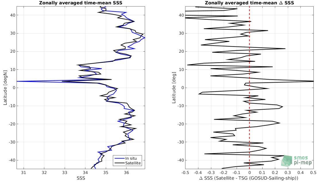
Figure 8: Left panel: Zonal mean SSS from SMOS SSS L3 v2 - Daily - 0.5 Deg (CATDS-CECOS-IFREMER) satellite product (black) and from TSG (GOSUD-Sailing-ship) (blue). Right panel: Zonal mean of \Delta SSS (Satellite - TSG (GOSUD-Sailing-ship)) for all the collected Pi-MEP match-up pairs estimated over the full satellite product period.
