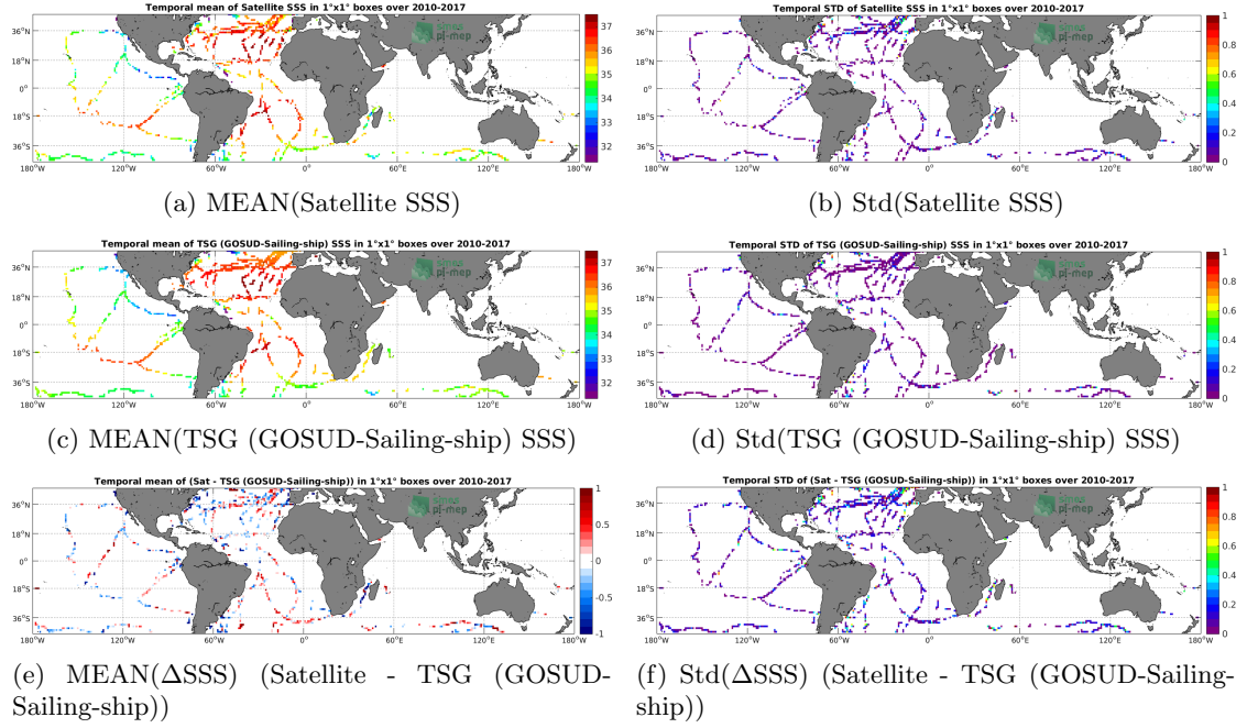
Figure 6: Temporal mean (left) and Std (right) of SSS from SMOS SSS L3 v2 - Daily - 0.5 Deg (CATDS-CECOS-IFREMER) (top), TSG (GOSUD-Sailing-ship) (middle), and of \Delta SSS (Satellite - TSG (GOSUD-Sailing-ship)). Only match-up pairs are used to generate these maps.
