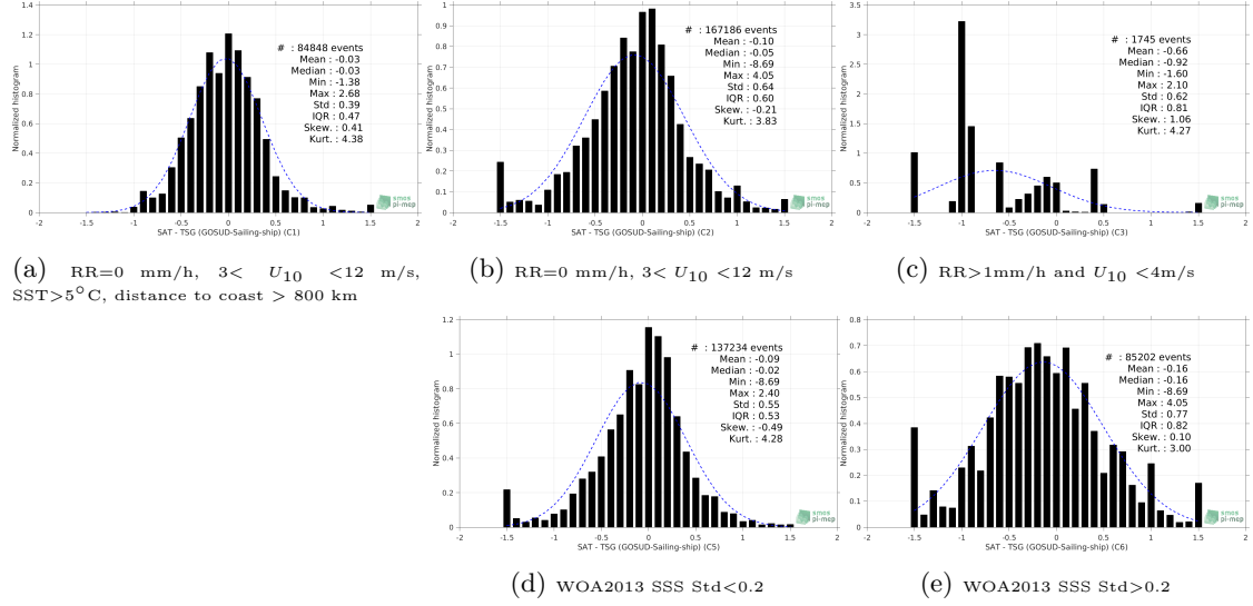
Figure 13: Normalized histogram of \Delta SSS (SMOS SSS L3 v2 - Daily - 0.5 Deg (CATDS-CECOS-IFREMER) - TSG (GOSUD-Sailing-ship)) for 5 different subdatasets corresponding to: RR=0 mm/h, 3 < U_{10} < 12 m/s, SST>5°C, distance to coast > 800 km (a), RR=0 mm/h, 3 < U_{10} < 12 m/s (b), RR>1mm/h and U_{10} < 4 m/s (c), WOA2013 SSS Std<0.2 (d), WOA2013 SSS Std>0.2 (e).
