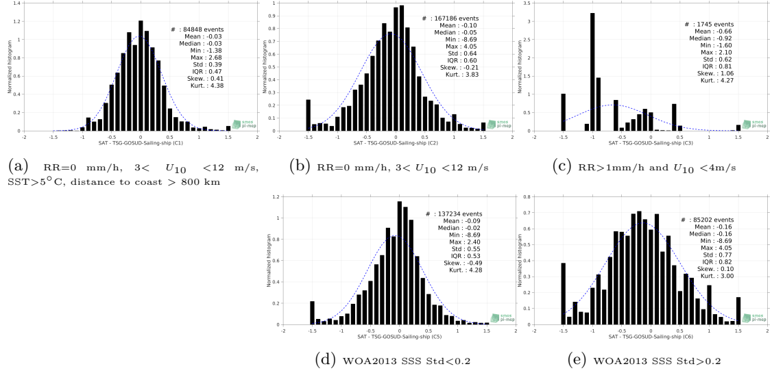
Figure 13: Normalized histogram of \Delta SSS (SMOS L3 v2 - Daily - 0.5 Deg (CATDS-CECOS-IFREMER) - TSG-GOSUD-Sailing-ship) for 5 different subdatasets corresponding to: RR=0 mm/h, 3 < U_{10} < 12 m/s, SST>5°C, distance to coast > 800 km (a), RR=0 mm/h, 3 < U_{10} < 12 m/s (b), RR>1mm/h and U_{10} < 4 m/s (c), WOA2013 SSS Std<0.2 (d), WOA2013 SSS Std>0.2 (e).
