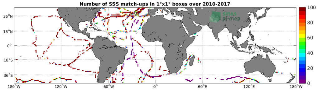
Figure 4: Number of SSS match-ups between TSG-GOSUD-Sailing-ship SSS and the SMOS L3 v2 - Daily - 0.5 Deg (CATDS-CECOS-IFREMER) SSS product for the Mid-Low Latitudes 45N-45S Pi-MEP region over 1^\circ \times 1^\circ boxes and for the full satellite product period.
