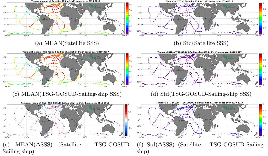
Figure 6: Temporal mean (left) and Std (right) of SSS from SMOS L3 v2 - Daily - 0.5 Deg (CATDS-CECOS-IFREMER) (top), TSG-GOSUD-Sailing-ship (middle), and of \Delta SSS (Satellite - TSG-GOSUD-Sailing-ship). Only match-up pairs are used to generate these maps.
