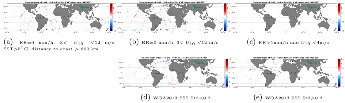
Figure 12: Temporal mean gridded over spatial boxes of size 1^\circ \times 1^\circ of \Delta SSS (SMOS L3 v2 - Daily - 0.5 Deg (CATDS-CECOS-IFREMER) - TSG-GOSUD-Sailing-ship) for 5 different subdatasets corresponding to: RR=0 mm/h, 3 < U_{10} < 12 m/s, SST > 5^\circ C , distance to coast > 800 km (a), RR=0 mm/h, 3 < U_{10} < 12 m/s (b), RR > 1 mm/h and U_{10} < 4 m/s (c), WOA2013 SSS Std < 0.2 (d), WOA2013 SSS Std > 0.2 (e).
