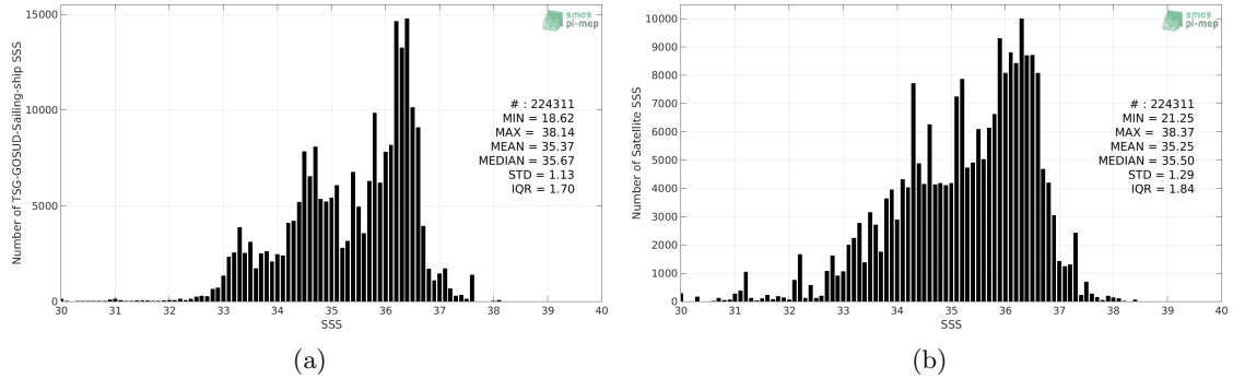
Figure 2: Histograms of SSS from TSG-GOSUD-Sailing-ship (a) and SMOS L3 v2 - Daily - 0.5 Deg (CATDS-CECOS-IFREMER) (b) considering all match-up pairs per bins of 0.1 over the Mid-Low Latitudes 45N-45S Pi-MEP region and for the full satellite product period.
