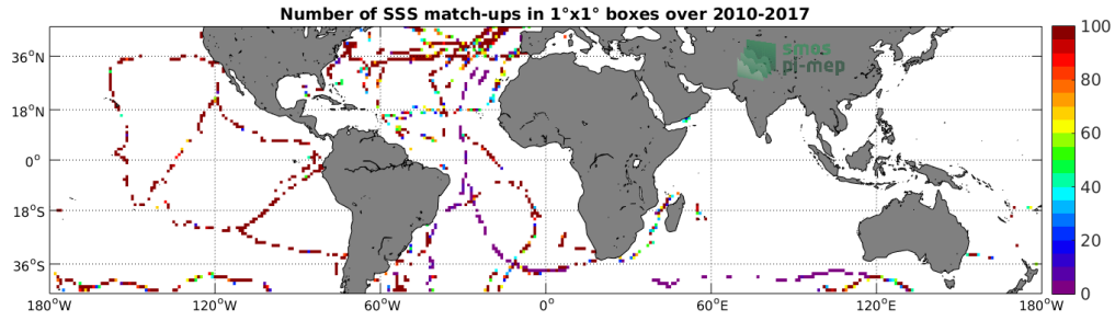
Figure 4: Number of SSS match-ups between TSG-GOSUD-Sailing-ship SSS and the SMOS-L3-CATDS-CECOS-IFREMER-V2-1DAY-0.5DEG SSS product for the Mid-Low Latitudes 45N-45S Pi-MEP region over 1^\circ \times 1^\circ boxes and for the full satellite product period.
