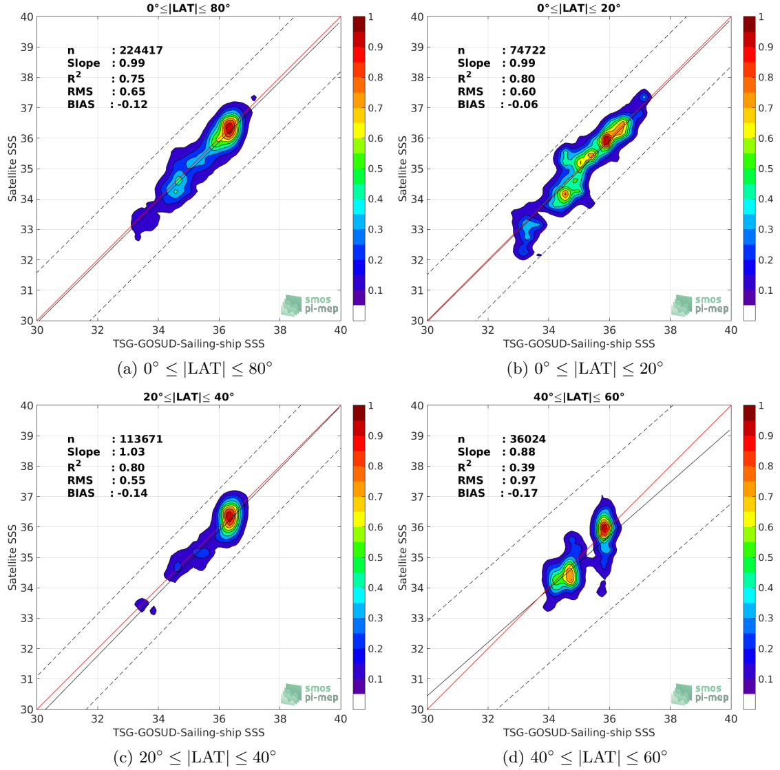
Figure 9: Contour maps of the concentration of SMOS-L3-CATDS-CECOS-IFREMER-V2-1DAY-0.5DEG SSS (y-axis) versus TSG-GOSUD-Sailing-ship SSS (x-axis) at match-up pairs for different latitude bands. For each plot, the red line shows x=y . The black thin and dashed lines indicate a linear fit through the data cloud and the \pm 95\% confidence levels, respectively. The number match-up pairs n , the slope and R^2 coefficient of the linear fit, the root mean square (RMS) and the mean bias between satellite and in situ data are indicated for each latitude band in each plots.
