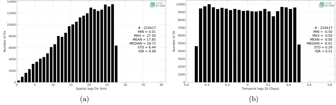
Figure 5: Histograms of the spatial (a) and temporal (b) lags between the time of the TSG-GOSUD-Sailing-ship measurements and the date of the corresponding SMOS-L3-CATDS-CECOS-IFREMER-V2-1DAY-0.5DEG SSS product.
