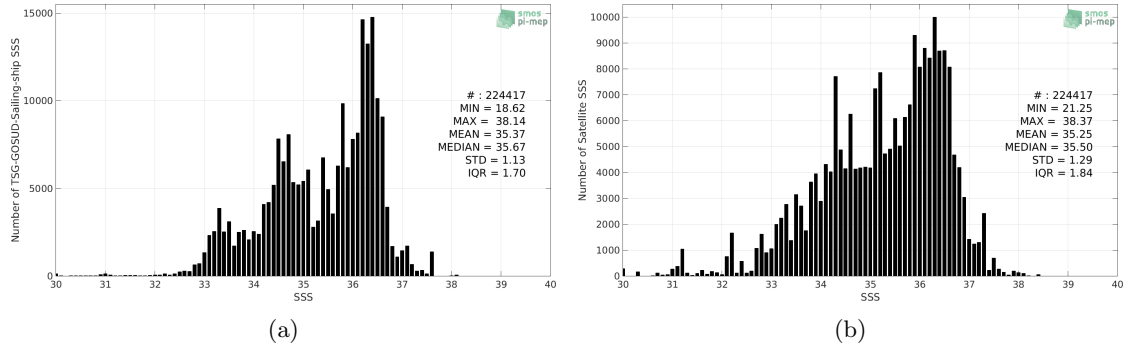
Figure 2: Histograms of SSS from TSG-GOSUD-Sailing-ship (a) and SMOS-L3-CATDS-CECOS-IFREMER-V2-1DAY-0.5DEG (b) considering all match-up pairs per bins of 0.1 over the Mid-Low Latitudes 45N-45S Pi-MEP region and for the full satellite product period.
