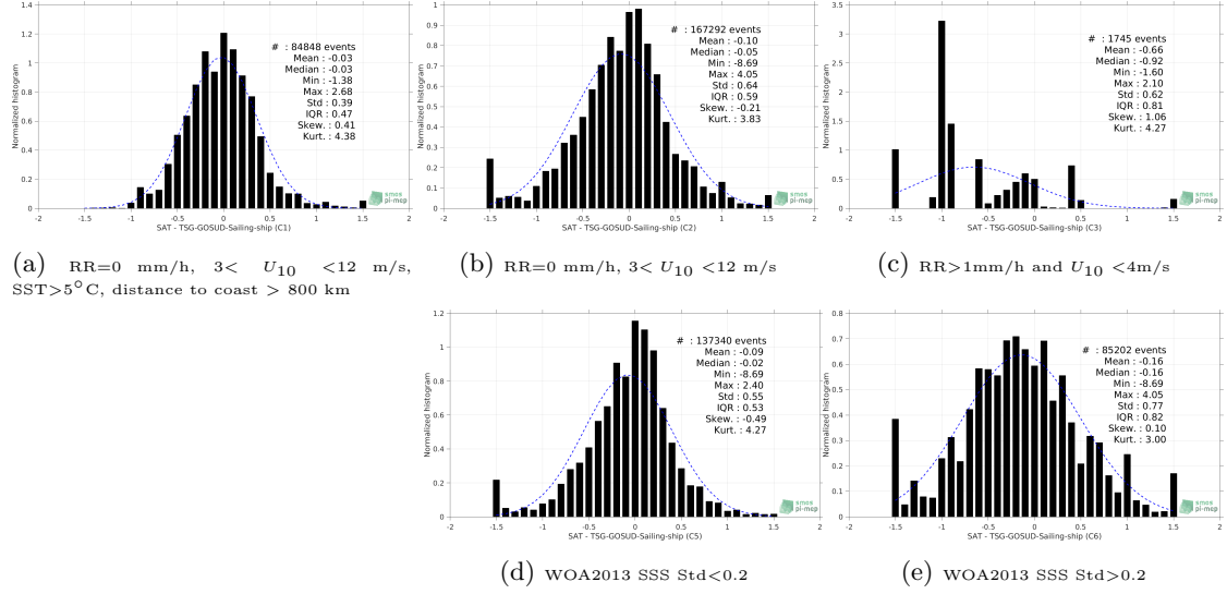
Figure 13: Normalized histogram of \Delta SSS (SMOS-L3-CATDS-CECOS-IFREMER-V2-1DAY-0.5DEG - TSG-GOSUD-Sailing-ship) for 5 different subdatasets corresponding to: RR=0 mm/h, 3 < U_{10} < 12 m/s, SST>5°C, distance to coast > 800 km (a), RR=0 mm/h, 3 < U_{10} < 12 m/s (b), RR>1 mm/h and U_{10} < 4 m/s (c), WOA2013 SSS Std<0.2 (d), WOA2013 SSS Std>0.2 (e).
