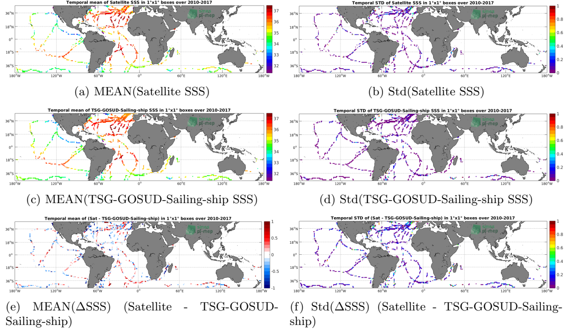
Figure 6: Temporal mean (left) and Std (right) of SSS from SMOS-L3-CATDS-CECOS-IFREMER-V2-1DAY-0.5DEG (top), TSG-GOSUD-Sailing-ship (middle), and of \Delta SSS (Satellite - TSG-GOSUD-Sailing-ship). Only match-up pairs are used to generate these maps.
