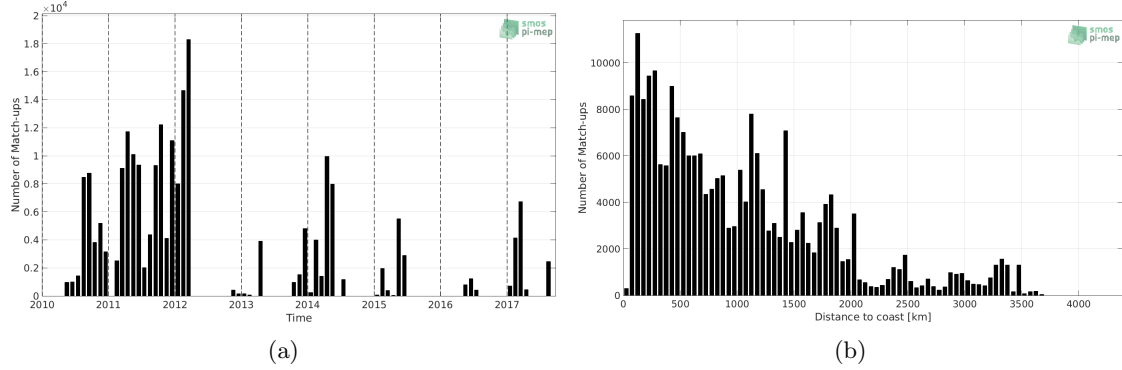
Figure 1: Number of match-ups between TSG-GOSUD-Sailing-ship and SMOS-L3-CATDS-CECOS-IFREMER-V2-1DAY-0.5DEG SSS as a function of time (a) and as function of the distance to coast (b) over the Mid-Low Latitudes 45N-45S Pi-MEP region and for the full satellite product period.
