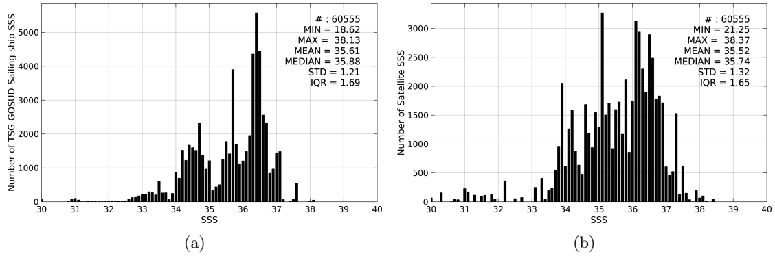
Figure 2: Histograms of SSS from TSG-GOSUD-Sailing-ship (a) and SMOS-L3-CATDS-CECOS-IFREMER-V2-1DAY-0.5DEG (b) considering all match-up pairs per bins of 0.1 over the Mid-Low Latitudes 45N-45S Pi-MEP region and for the full satellite product period.
