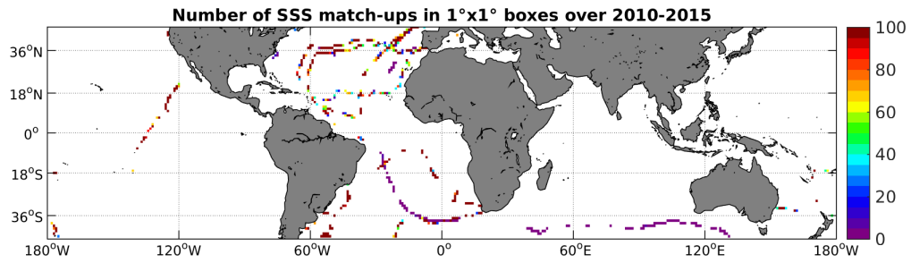
Figure 4: Number of SSS match-ups between TSG-GOSUD-Sailing-ship SSS and the SMOS-L3-CATDS-CECOS-IFREMER-V2-1DAY-0.5deg SSS product for the Mid-Low Latitudes 45N-45S Pi-MEP region over 1°x1° boxes and for the full satellite product period.
