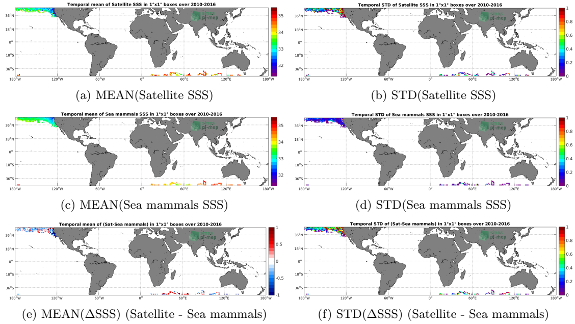
Figure 6: Temporal mean (left) and STD (right) of SSS from SMOS-L3-CATDS-CECOS-IFREMER-V2-1DAY-0.5DEG (top), Sea mammals (middle), and of \Delta SSS (Satellite - Sea mammals). Only match-up pairs are used to generate these maps.
