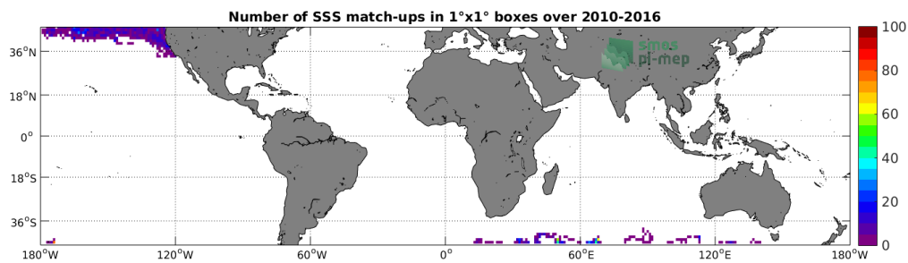
Figure 4: Number of SSS match-ups between Sea mammals SSS and the SMOS-L3-CATDS-CECOS-IFREMER-V2-1DAY-0.5DEG SSS product for the Mid-Low Latitudes 45N-45S Pi-MEP region over 1^\circ \times 1^\circ boxes and for the full satellite product period.
