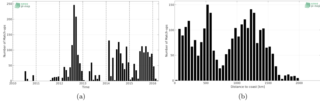
Figure 1: Number of match-ups between Sea mammals and SMOS-L3-CATDS-CECOS-IFREMER-V2-1DAY-0.5DEG SSS as a function of time (a) and as function of the distance to coast (b) over the Mid-Low Latitudes 45N-45S Pi-MEP region and for the full satellite product period.
