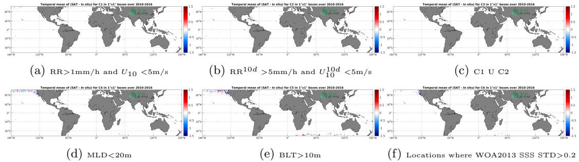
Figure 12: Temporal mean gridded over spatial boxes of size 1°x1° of \Delta SSS (SMOS-L3-CATDS-CECOS-IFREMER-V2-1DAY-0.5DEG - Sea mammals) for 6 different subdatasets corresponding to:RR>1mm/h and U_{10} < 5m/s (a), RR^{10d} > 5mm/h and U_{10}^{10d} < 5m/s (b), C1 U C2 (c),MLD<20m (d),BLT>10m (e),Locations where WOA2013 SSS STD>0.2 (f).
