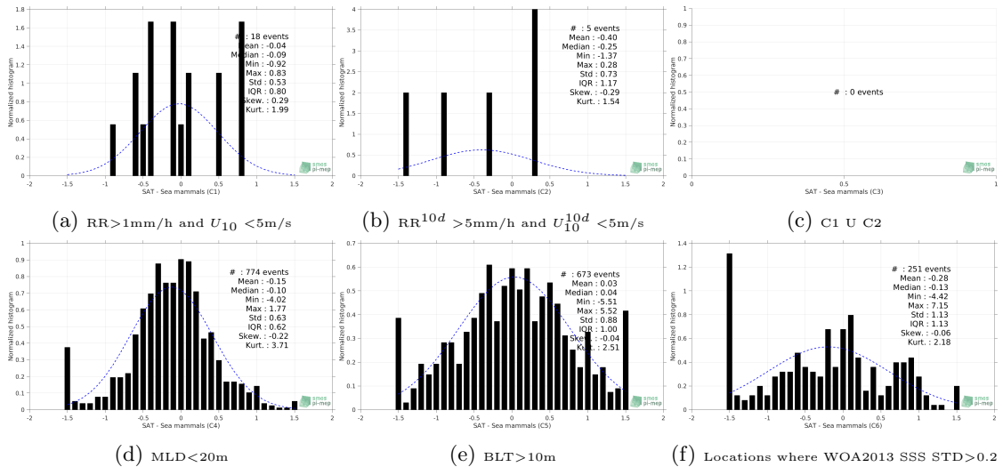
Figure 13: Normalized histogram of \Delta SSS (SMOS-L3-CATDS-CECOS-IFREMER-V2-1DAY-0.5DEG - Sea mammals) for 6 different subdatasets corresponding to: RR>1mm/h and U_{10} < 5m/s (a), RR^{10d} > 5mm/h and U_{10}^{10d} < 5m/s (b), C1 U C2 (c),MLD<20m (d),BLT>10m (e),Locations where WOA2013 SSS STD>0.2 (f).
