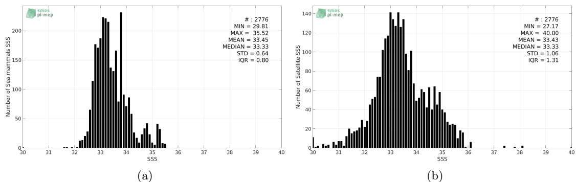
Figure 2: Histograms of SSS from Sea mammals (a) and SMOS-L3-CATDS-CECOS-IFREMER-V2-1DAY-0.5DEG (b) considering all match-up pairs per bins of 0.1 over the Mid-Low Latitudes 45N-45S Pi-MEP region and for the full satellite product period.
