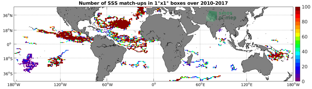
Figure 3: Number of SSS match-ups between Surface drifters SSS and the SMOS SSS L3 v2 - Daily - 0.5 Deg (CATDS-CECOS-IFREMER) SSS product for the Mid-Low Latitudes 45N-45S Pi-MEP region over 1^\circ \times 1^\circ boxes and for the full satellite product period.
