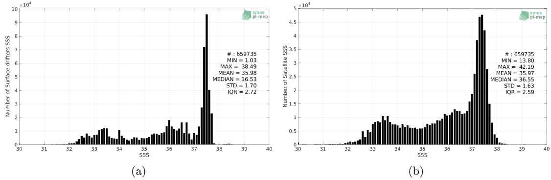
Figure 2: Histograms of SSS from Surface drifters (a) and SMOS SSS L3 v2 - Daily - 0.5 Deg (CATDS-CECOS-IFREMER) (b) considering all match-up pairs per bins of 0.1 over the Mid-Low Latitudes 45N-45S Pi-MEP region and for the full satellite product period.
