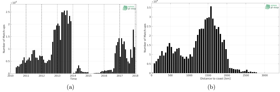
Figure 1: Number of match-ups between Surface drifters and SMOS SSS L3 v2 - Daily - 0.5 Deg (CATDS-CECOS-IFREMER) SSS as a function of time (a) and as function of the distance to coast (b) over the Mid-Low Latitudes 45N-45S Pi-MEP region and for the full satellite product period.
