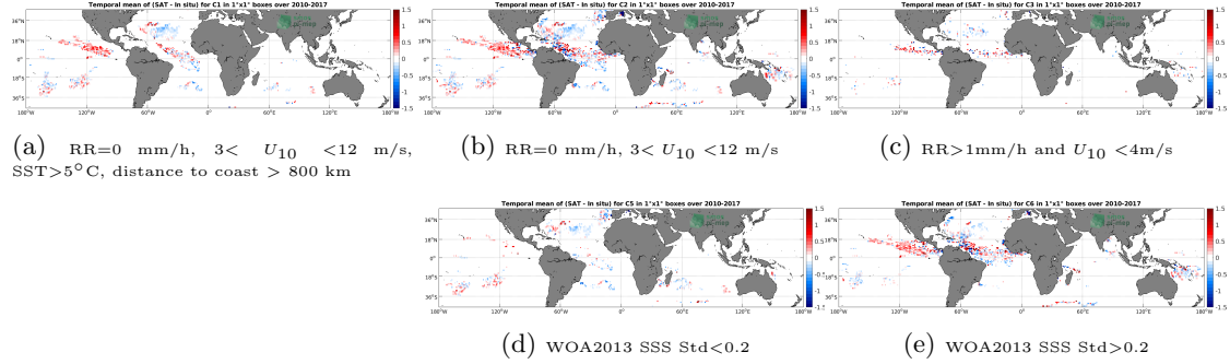
Figure 11: Temporal mean gridded over spatial boxes of size 1^\circ \times 1^\circ of \Delta SSS (SMOS SSS L3 v2 - Daily - 0.5 Deg (CATDS-CECOS-IFREMER) - Surface drifters) for 5 different subdatasets corresponding to: RR=0 mm/h, 3 < U_{10} < 12 m/s, SST > 5^\circ\text{C} , distance to coast > 800 km (a), RR=0 mm/h, 3 < U_{10} < 12 m/s (b), RR > 1 mm/h and U_{10} < 4 m/s (c), WOA2013 SSS Std < 0.2 (d), WOA2013 SSS Std > 0.2 (e).
