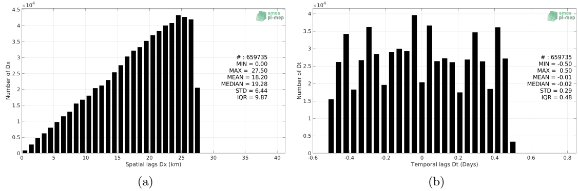
Figure 4: Histograms of the spatial (a) and temporal (b) lags between the location/time of the Surface drifters measurement and the date of the corresponding SMOS SSS L3 v2 - Daily - 0.5 Deg (CATDS-CECOS-IFREMER) SSS pixel.
