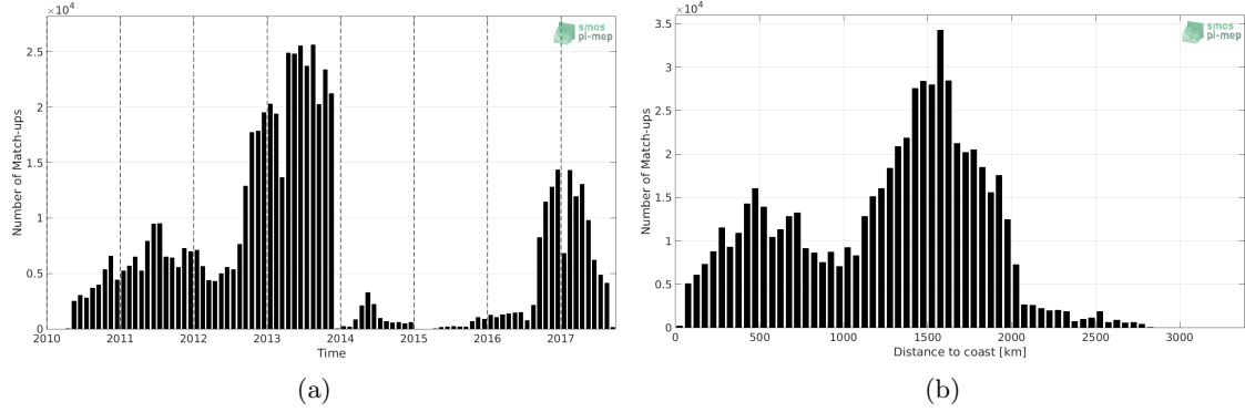
Figure 1: Number of match-ups between Surface drifters and SMOS L3 v2 - Daily - 0.5 Deg (CATDS-CECOS-IFREMER) SSS as a function of time (a) and as function of the distance to coast (b) over the Mid-Low Latitudes 45N-45S Pi-MEP region and for the full satellite product period.
