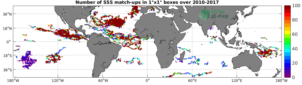
Figure 3: Number of SSS match-ups between Surface drifters SSS and the SMOS L3 v2 - Daily - 0.5 Deg (CATDS-CECOS-IFREMER) SSS product for the Mid-Low Latitudes 45N-45S Pi-MEP region over 1°x1° boxes and for the full satellite product period.
