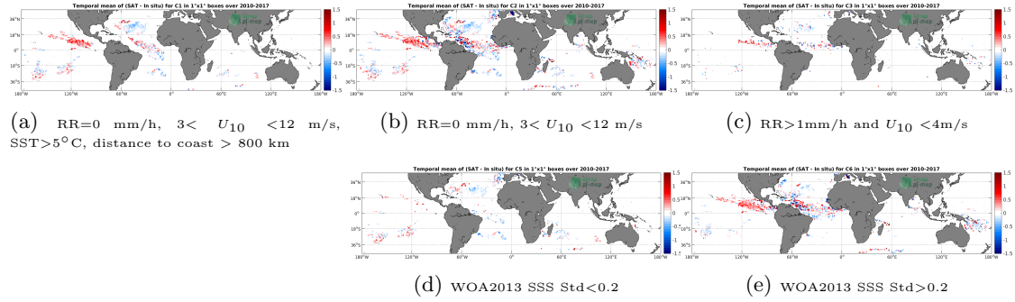
Figure 11: Temporal mean gridded over spatial boxes of size 1^\circ \times 1^\circ of \Delta SSS (SMOS L3 v2 - Daily - 0.5 Deg (CATDS-CECOS-IFREMER) - Surface drifters) for 5 different subdatasets corresponding to: RR=0 mm/h, 3 < U_{10} < 12 m/s, SST > 5^\circ C , distance to coast > 800 km (a), RR=0 mm/h, 3 < U_{10} < 12 m/s (b), RR > 1 mm/h and U_{10} < 4 m/s (c), WOA2013 SSS Std < 0.2 (d), WOA2013 SSS Std > 0.2 (e).
