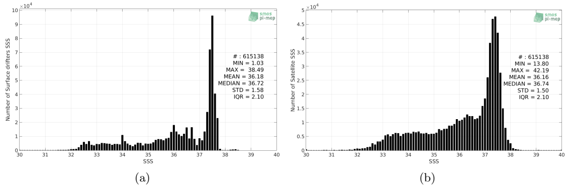
Figure 2: Histograms of SSS from Surface drifters (a) and SMOS L3 v2 - Daily - 0.5 Deg (CATDS-CECOS-IFREMER) (b) considering all match-up pairs per bins of 0.1 over the Mid-Low Latitudes 45N-45S Pi-MEP region and for the full satellite product period.
