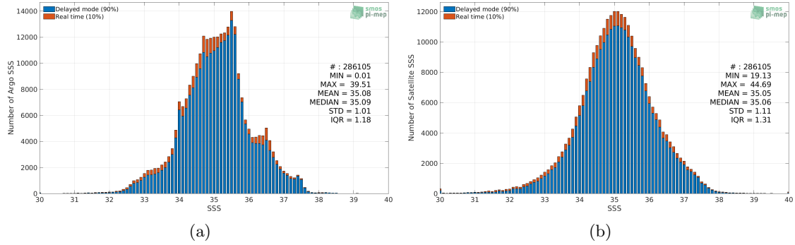
Figure 2: Histograms of SSS from Argo (a) and SMOS SSS L3 v2 - Daily - 0.5 Deg (CATDS-CECOS-IFREMER) (b) considering all match-up pairs per bins of 0.1 over the Mid-Low Latitudes 45N-45S Pi-MEP region and for the full satellite product period.
