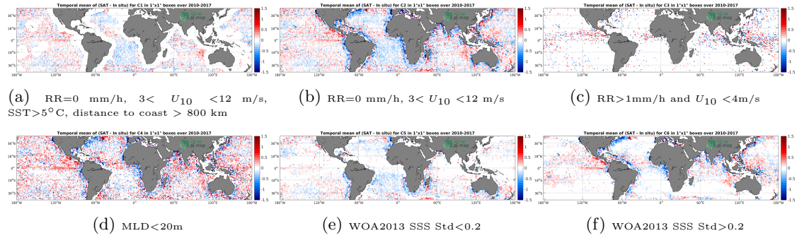
Figure 12: Temporal mean gridded over spatial boxes of size 1^\circ \times 1^\circ of \Delta SSS (SMOS SSS L3 v2 - Daily - 0.5 Deg (CATDS-CECOS-IFREMER) - Argo) for 6 different subdatasets corresponding to: RR=0 mm/h, 3 < U_{10} < 12 m/s, SST > 5^\circ C , distance to coast > 800 km (a), RR=0 mm/h, 3 < U_{10} < 12 m/s (b), RR > 1 mm/h and U_{10} < 4 m/s (c), MLD < 20 m (d), WOA2013 SSS Std < 0.2 (e), WOA2013 SSS Std > 0.2 (f).
