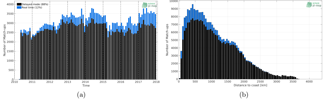
Figure 1: Number of match-ups between Argo and SMOS SSS L3 v2 - Daily - 0.5 Deg (CATDS-CECOS-IFREMER) SSS as a function of time (a) and as function of the distance to coast (b) over the Mid-Low Latitudes 45N-45S Pi-MEP region and for the full satellite product period.
