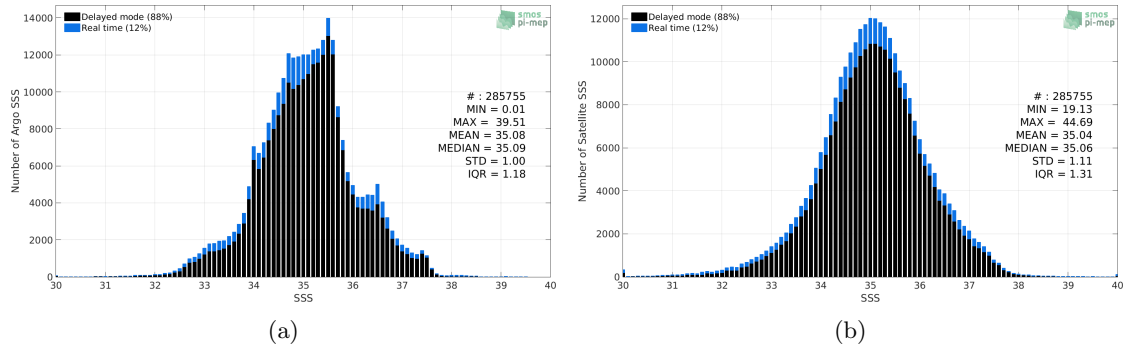
Figure 2: Histograms of SSS from Argo (a) and SMOS SSS L3 v2 - Daily - 0.5 Deg (CATDS-CECOS-IFREMER) (b) considering all match-up pairs per bins of 0.1 over the Mid-Low Latitudes 45N-45S Pi-MEP region and for the full satellite product period.
