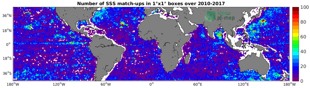
Figure 4: Number of SSS match-ups between Argo SSS and the SMOS SSS L3 v2 - Daily - 0.5 Deg (CATDS-CECOS-IFREMER) SSS product for the Mid-Low Latitudes 45N-45S Pi-MEP region over 1^\circ \times 1^\circ boxes and for the full satellite product period.
