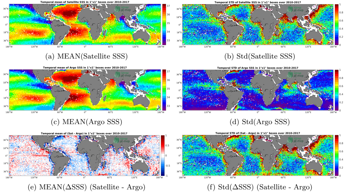
Figure 6: Temporal mean (left) and Std (right) of SSS from SMOS SSS L3 v2 - Daily - 0.5 Deg (CATDS-CECOS-IFREMER) (top), Argo (middle), and of \Delta SSS (Satellite - Argo). Only match-up pairs are used to generate these maps.
