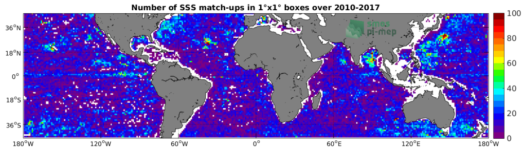
Figure 4: Number of SSS match-ups between Argo SSS and the SMOS L3 v2 - Daily - 0.5 Deg (CATDS-CECOS-IFREMER) SSS product for the Mid-Low Latitudes 45N-45S Pi-MEP region over 1^\circ \times 1^\circ boxes and for the full satellite product period.
