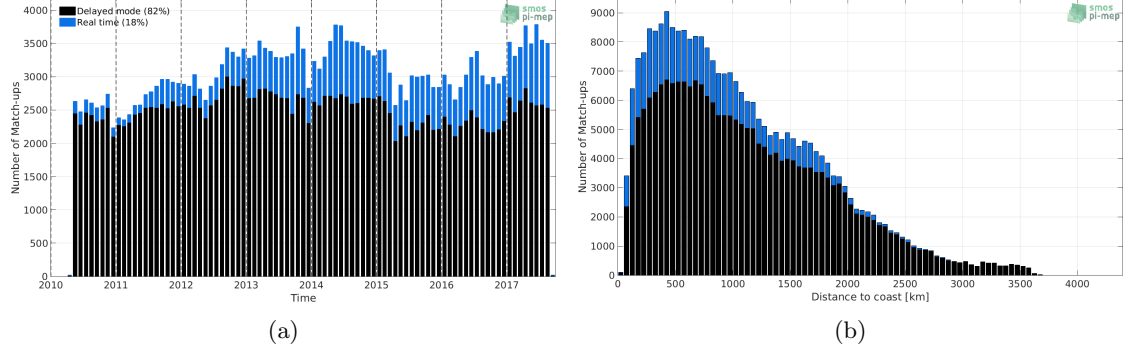
Figure 1: Number of match-ups between Argo and SMOS L3 v2 - Daily - 0.5 Deg (CATDS-CECOS-IFREMER) SSS as a function of time (a) and as function of the distance to coast (b) over the Mid-Low Latitudes 45N-45S Pi-MEP region and for the full satellite product period.
