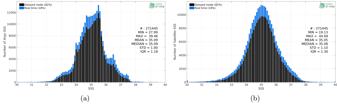
Figure 2: Histograms of SSS from Argo (a) and SMOS L3 v2 - Daily - 0.5 Deg (CATDS-CECOS-IFREMER) (b) considering all match-up pairs per bins of 0.1 over the Mid-Low Latitudes 45N-45S Pi-MEP region and for the full satellite product period.
