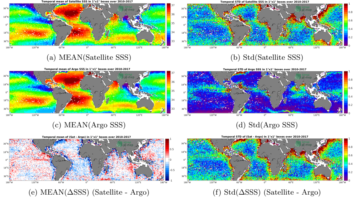
Figure 6: Temporal mean (left) and Std (right) of SSS from SMOS L3 v2 - Daily - 0.5 Deg (CATDS-CECOS-IFREMER) (top), Argo (middle), and of \Delta SSS (Satellite - Argo). Only match-up pairs are used to generate these maps.
