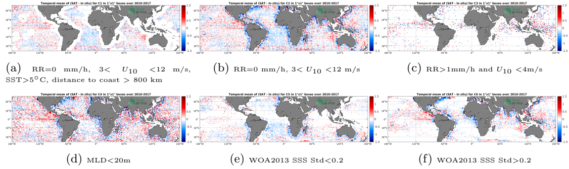
Figure 12: Temporal mean gridded over spatial boxes of size 1^\circ \times 1^\circ of \Delta SSS (SMOS L3 v2 - Daily - 0.5 Deg (CATDS-CECOS-IFREMER) - Argo) for 6 different subdatasets corresponding to: RR=0 mm/h, 3 < U_{10} < 12 m/s, SST > 5^\circ C , distance to coast > 800 km (a), RR=0 mm/h, 3 < U_{10} < 12 m/s (b), RR > 1 mm/h and U_{10} < 4 m/s (c), MLD < 20 m (d), WOA2013 SSS Std < 0.2 (e), WOA2013 SSS Std > 0.2 (f).
