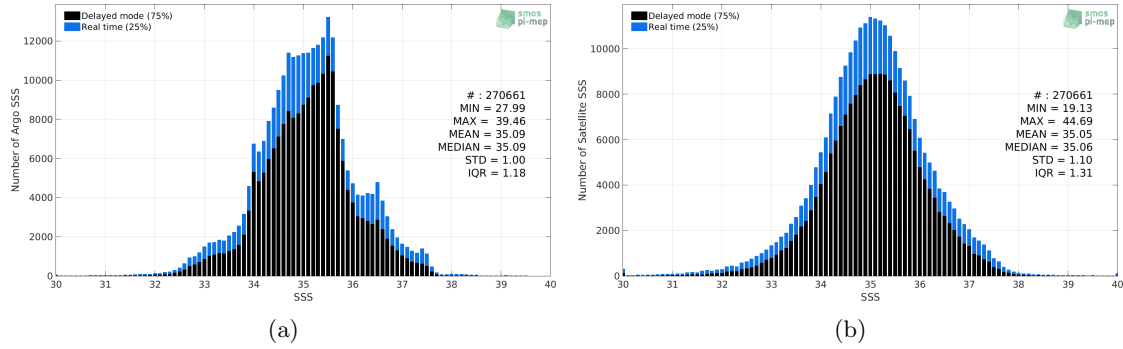
Figure 2: Histograms of SSS from Argo (a) and SMOS-L3-CATDS-CECOS-IFREMER-V2-1DAY-0.5DEG (b) considering all match-up pairs per bins of 0.1 over the Mid-Low Latitudes 45N-45S Pi-MEP region and for the full satellite product period.
