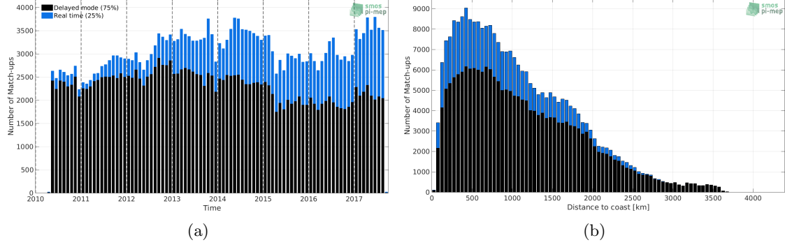
Figure 1: Number of match-ups between Argo and SMOS-L3-CATDS-CECOS-IFREMER-V2-1DAY-0.5DEG SSS as a function of time (a) and as function of the distance to coast (b) over the Mid-Low Latitudes 45N-45S Pi-MEP region and for the full satellite product period.
