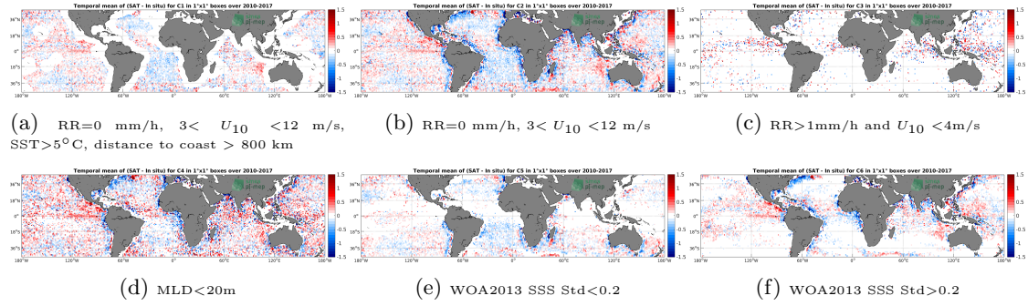
Figure 12: Temporal mean gridded over spatial boxes of size 1^\circ \times 1^\circ of \Delta SSS (SMOS-L3-CATDS-CECOS-IFREMER-V2-1DAY-0.5DEG - Argo) for 6 different subdatasets corresponding to: RR=0 mm/h, 3 < U_{10} < 12 m/s, SST > 5^\circ C , distance to coast > 800 km (a), RR=0 mm/h, 3 < U_{10} < 12 m/s (b), RR > 1 mm/h and U_{10} < 4 m/s (c), MLD < 20 m (d), WOA2013 SSS Std < 0.2 (e), WOA2013 SSS Std > 0.2 (f).
