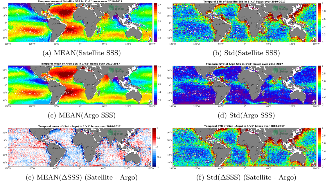
Figure 6: Temporal mean (left) and Std (right) of SSS from SMOS-L3-CATDS-CECOS-IFREMER-V2-1DAY-0.5DEG (top), Argo (middle), and of \Delta SSS (Satellite - Argo). Only match-up pairs are used to generate these maps.
