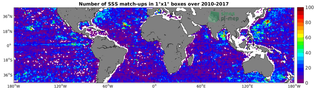
Figure 4: Number of SSS match-ups between Argo SSS and the SMOS-L3-CATDS-CECOS-IFREMER-V2-1DAY-0.5DEG SSS product for the Mid-Low Latitudes 45N-45S Pi-MEP region over 1^\circ \times 1^\circ boxes and for the full satellite product period.
