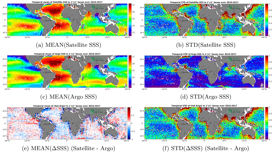
Figure 6: Temporal mean (left) and STD (right) of SSS from SMOS-L3-CATDS-CECOS-IFREMER-V2-1DAY-0.5DEG (top), Argo (middle), and of \Delta SSS (Satellite - Argo). Only match-up pairs are used to generate these maps.
