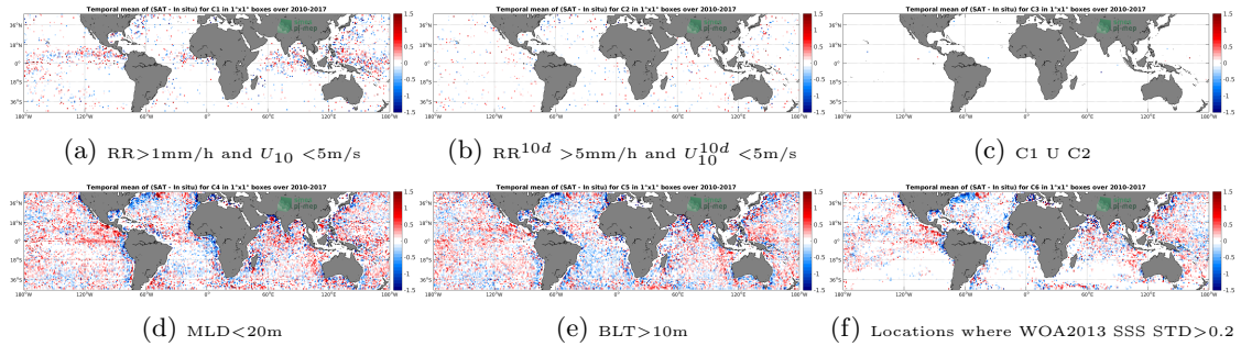
Figure 12: Temporal mean gridded over spatial boxes of size 1°x1° of \Delta SSS (SMOS-L3-CATDS-CECOS-IFREMER-V2-1DAY-0.5DEG - Argo) for 6 different subdatasets corresponding to:RR>1mm/h and U_{10} < 5m/s (a), RR^{10d} > 5mm/h and U_{10}^{10d} < 5m/s (b), C1 U C2 (c),MLD<20m (d),BLT>10m (e),Locations where WOA2013 SSS STD>0.2 (f).
