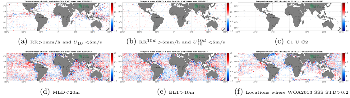
Figure 12: Temporal mean gridded over spatial boxes of size 1^\circ \times 1^\circ of \Delta\text{SSS} (SMOS-L3-CATDS-CECOS-IFREMER-V2-1DAY-0.5DEG - Argo) for 6 different subdatasets corresponding to: \text{RR}>1\text{mm/h} and U_{10}<5\text{m/s} (a), \text{RR}^{10d}>5\text{mm/h} and U_{10}^{10d}<5\text{m/s} (b), C1 U C2 (c), \text{MLD}<20\text{m} (d), \text{BLT}>10\text{m} (e), Locations where WOA2013 SSS STD >0.2 (f).
