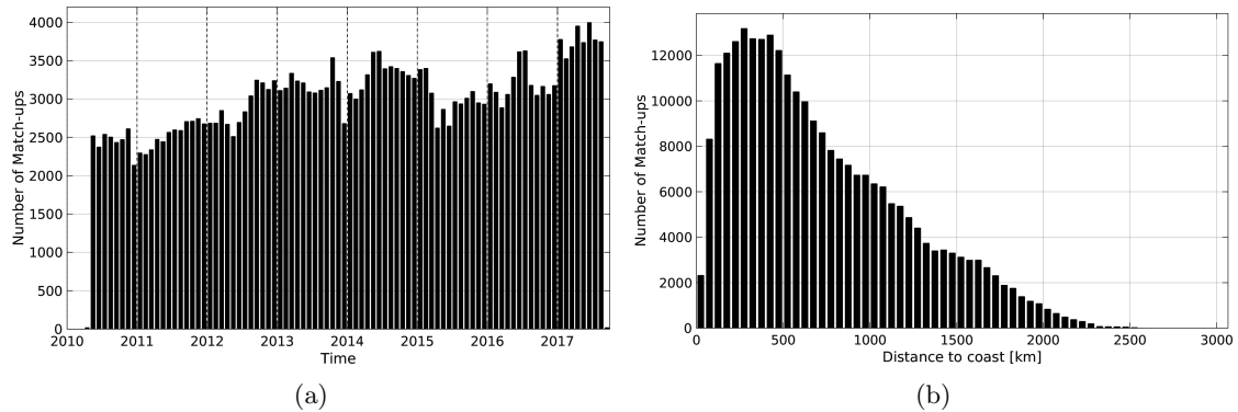
Figure 1: Number of match-ups between Argo and SMOS-L3-CATDS-CECOS-IFREMER-V2-1DAY-0.5DEG SSS as a function of time (a) and as function of the distance to coast (b) over the Mid-Low Latitudes 45N-45S Pi-MEP region and for the full satellite product period.
