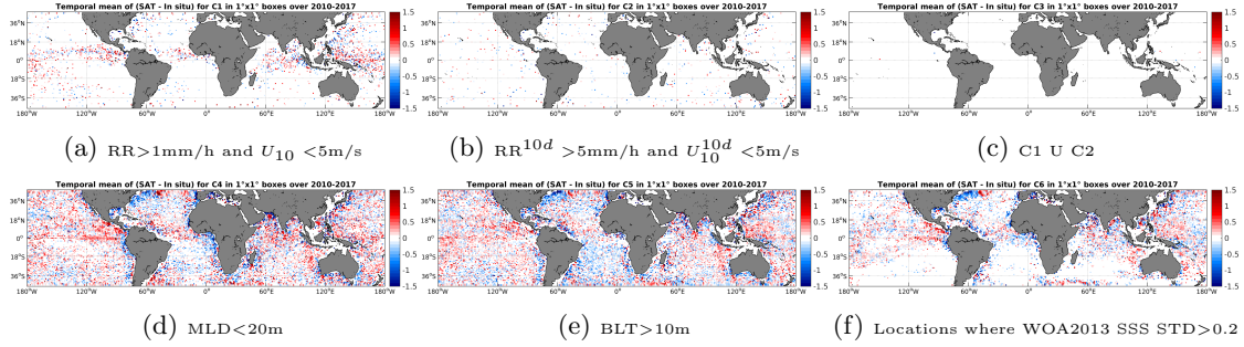
Figure 12: Temporal mean gridded over spatial boxes of size 1^\circ \times 1^\circ of \Delta SSS (SMOS-L3-CATDS-CECOS-IFREMER-V2-1DAY-0.5DEG - Argo) for 6 different subdatasets corresponding to: RR>1\text{mm/h} and U_{10}<5\text{m/s} (a), RR^{10d}>5\text{mm/h} and U_{10}^{10d}<5\text{m/s} (b), C1 U C2 (c), MLD<20\text{m} (d), BLT>10\text{m} (e), Locations where WOA2013 SSS STD>0.2 (f).
