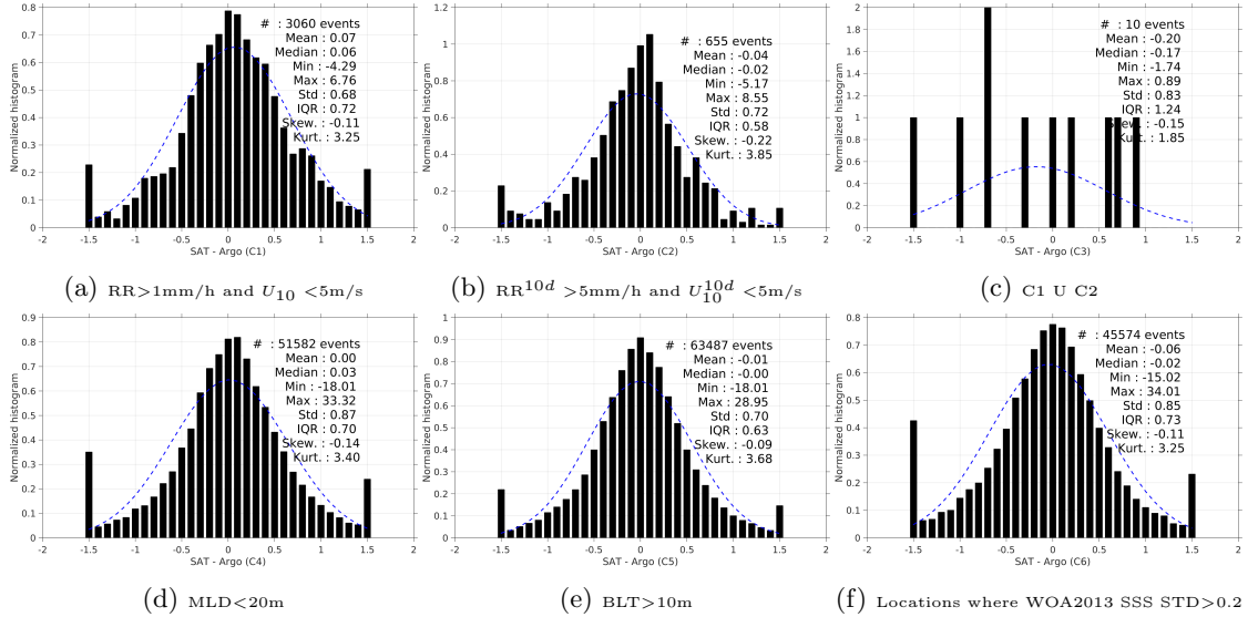
Figure 13: Normalized histogram of \Delta SSS (SMOS-L3-CATDS-CECOS-IFREMER-V2-1DAY-0.5DEG - Argo) for 6 different subdatasets corresponding to: RR>1\text{mm/h} and U_{10}<5\text{m/s} (a), RR^{10d}>5\text{mm/h} and U_{10}^{10d}<5\text{m/s} (b), C1 U C2 (c), MLD<20\text{m} (d), BLT>10\text{m} (e), Locations where WOA2013 SSS STD>0.2 (f).
