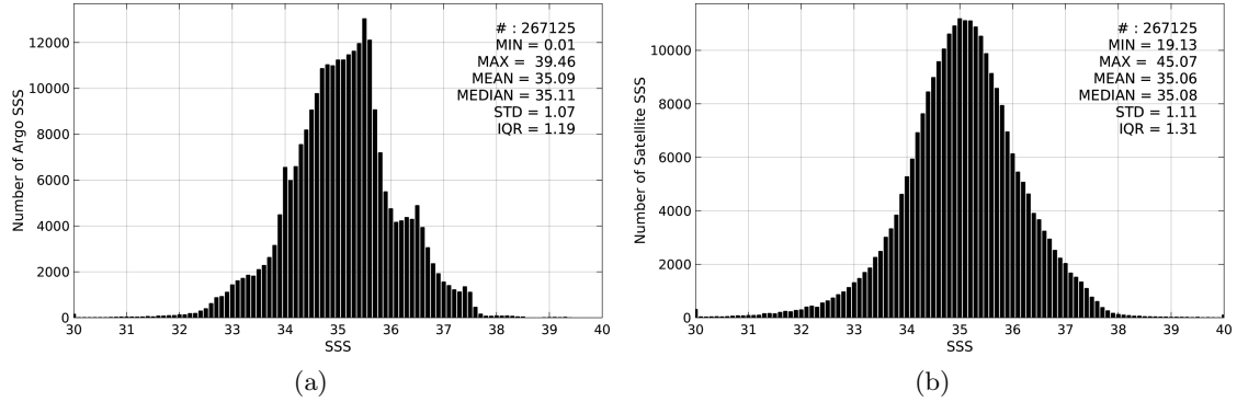
Figure 2: Histograms of SSS from Argo (a) and SMOS-L3-CATDS-CECOS-IFREMER-V2-1DAY-0.5DEG (b) considering all match-up pairs per bins of 0.1 over the Mid-Low Latitudes 45N-45S Pi-MEP region and for the full satellite product period.
