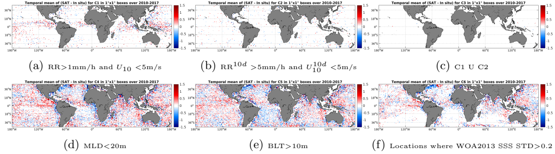
Figure 12: Temporal mean gridded over spatial boxes of size 1^\circ \times 1^\circ of \Delta SSS (SMOS-L3-CATDS-CECOS-IFREMER-V2-1DAY-0.5deg - Argo) for 6 different subdatasets corresponding to: RR > 1\text{mm/h} and U_{10} < 5\text{m/s} (a), RR^{10d} > 5\text{mm/h} and U_{10}^{10d} < 5\text{m/s} (b), C1 U C2 (c), MLD < 20\text{m} (d), BLT > 10\text{m} (e), Locations where WOA2013 SSS STD > 0.2 (f).
