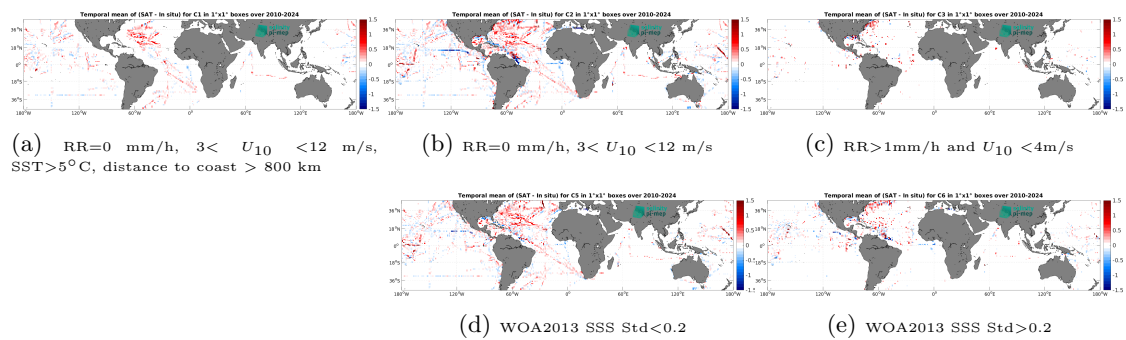
Figure 14: Temporal mean gridded over spatial boxes of size 1^\circ \times 1^\circ of \Delta SSS (SMOS SSS L3 v335 - Monthly - 25 km (CATDS-CPDC) - TSG (SAMOS)) for 5 different subdatasets corresponding to:RR=0 mm/h, 3 < U_{10} < 12 m/s, SST > 5^\circ\text{C} , distance to coast > 800 km (a), RR=0 mm/h, 3 < U_{10} < 12 m/s (b), RR > 1 mm/h and U_{10} < 4 m/s (c), WOA2013 SSS Std < 0.2 (d), WOA2013 SSS Std > 0.2 (e).
