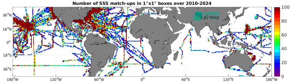
Figure 5: Number of SSS match-ups between TSG (SAMOS) SSS and the SMOS SSS L3 v335 - Monthly - 25 km (CATDS-CPDC) SSS product for the Mid-Low Latitudes 45N-45S Pi-MEP region over 1^\circ \times 1^\circ boxes and for the full satellite product period.
