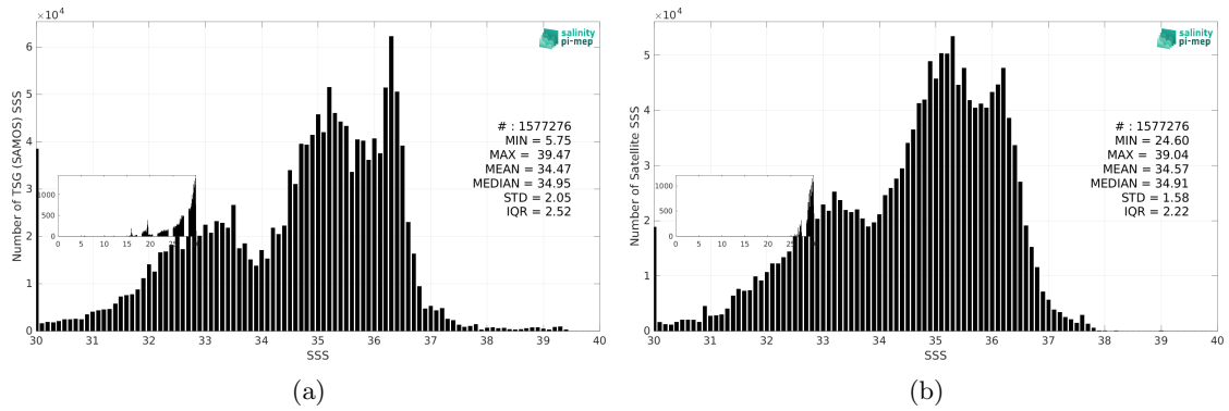
Figure 3: Histograms of SSS from TSG (SAMOS) (a) and SMOS SSS L3 v335 - Monthly - 25 km (CATDS-CPDC) (b) considering all match-up pairs per bins of 0.1 over the Mid-Low Latitudes 45N-45S Pi-MEP region and for the full satellite product period.
