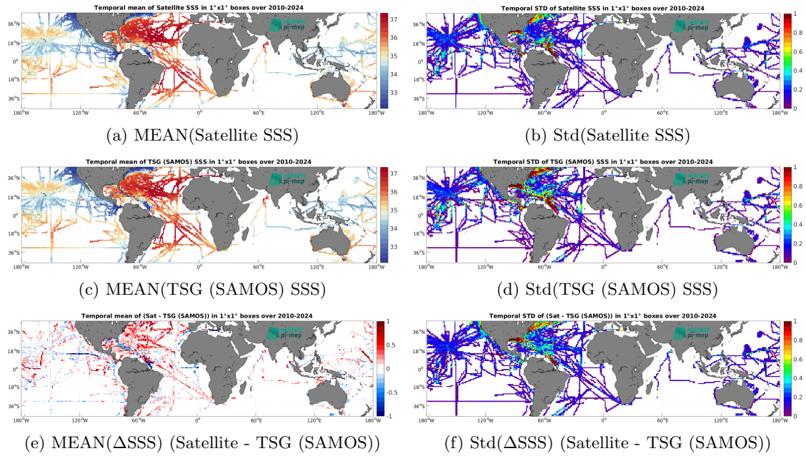
Figure 7: Temporal mean (left) and Std (right) of SSS from SMOS SSS L3 v335 - Monthly - 25 km (CATDS-CPDC) (top), TSG (SAMOS) (middle), and of \Delta SSS (Satellite - TSG (SAMOS)). Only match-up pairs are used to generate these maps.
