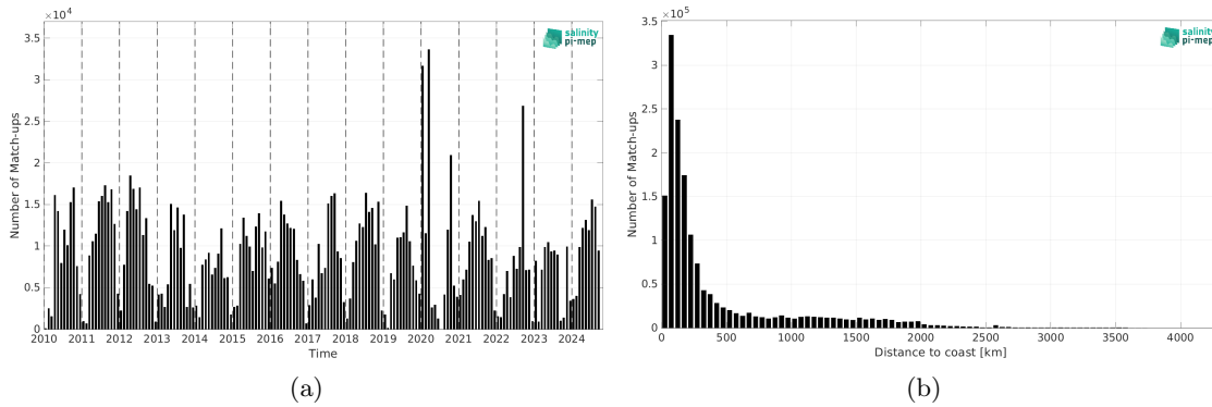
Figure 2: Number of match-ups between TSG (SAMOS) and SMOS SSS L3 v335 - Monthly - 25 km (CATDS-CPDC) SSS as a function of time (a) and as function of the distance to coast (b) over the Mid-Low Latitudes 45N-45S Pi-MEP region and for the full satellite product period.
