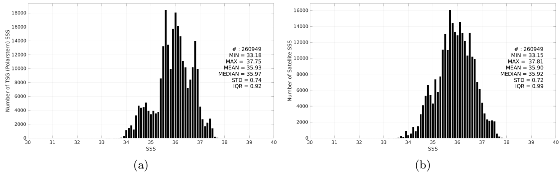
Figure 3: Histograms of SSS from TSG (Polarstern) (a) and SMOS SSS L3 v335 - Monthly - 25 km (CATDS-CPDC) (b) considering all match-up pairs per bins of 0.1 over the Mid-Low Latitudes 45N-45S Pi-MEP region and for the full satellite product period.
