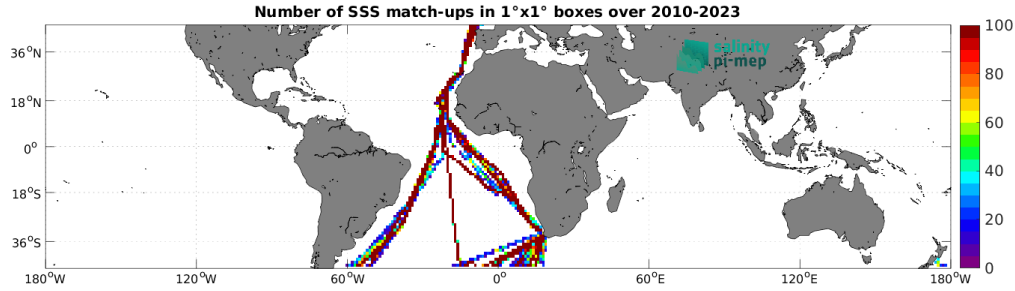
Figure 5: Number of SSS match-ups between TSG (Polarstern) SSS and the SMOS SSS L3 v335 - Monthly - 25 km (CATDS-CPDC) SSS product for the Mid-Low Latitudes 45N-45S Pi-MEP region over 1^\circ \times 1^\circ boxes and for the full satellite product period.
