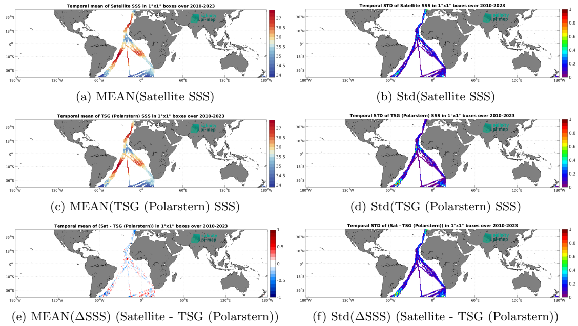
Figure 7: Temporal mean (left) and Std (right) of SSS from SMOS SSS L3 v335 - Monthly - 25 km (CATDS-CPDC) (top), TSG (Polarstern) (middle), and of \Delta SSS (Satellite - TSG (Polarstern)). Only match-up pairs are used to generate these maps.
