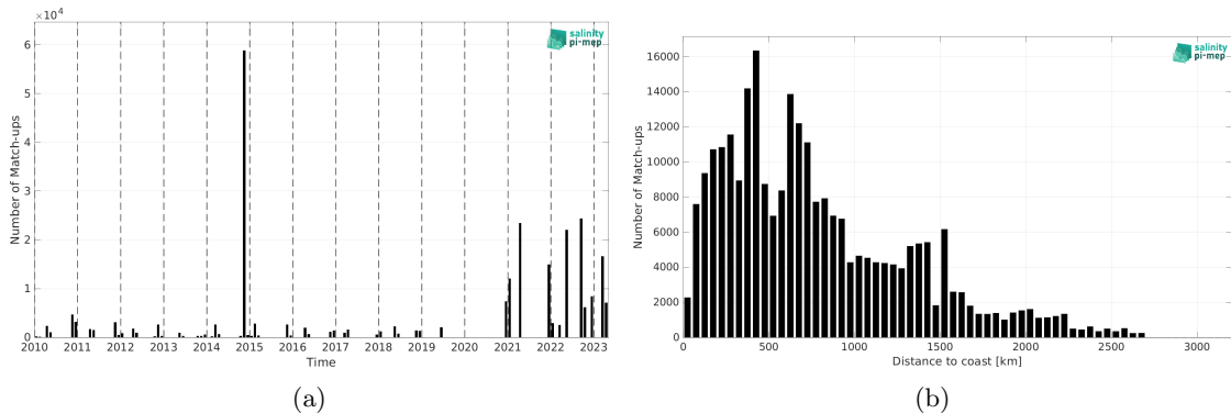
Figure 2: Number of match-ups between TSG (Polarstern) and SMOS SSS L3 v335 - Monthly - 25 km (CATDS-CPDC) SSS as a function of time (a) and as function of the distance to coast (b) over the Mid-Low Latitudes 45N-45S Pi-MEP region and for the full satellite product period.
