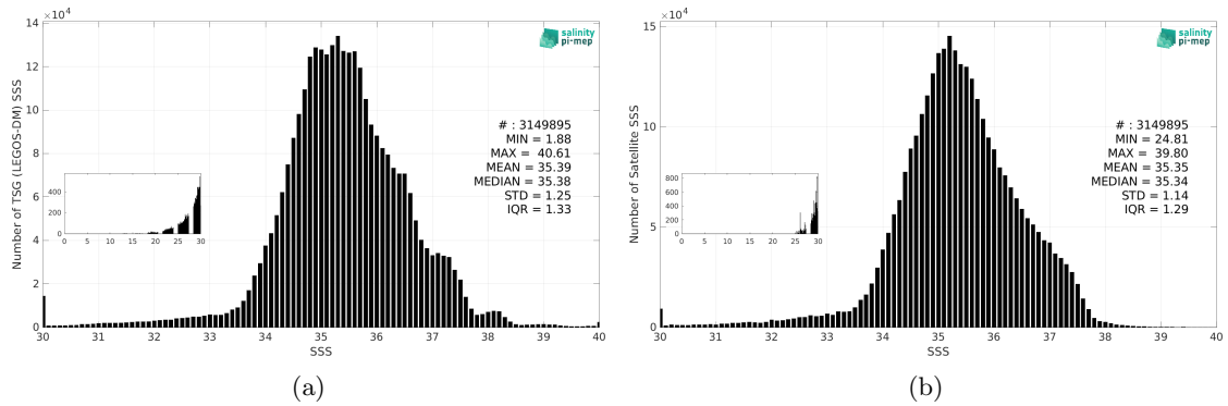
Figure 3: Histograms of SSS from TSG (LEGOS-DM) (a) and SMOS SSS L3 v335 - Monthly - 25 km (CATDS-CPDC) (b) considering all match-up pairs per bins of 0.1 over the Mid-Low Latitudes 45N-45S Pi-MEP region and for the full satellite product period.
