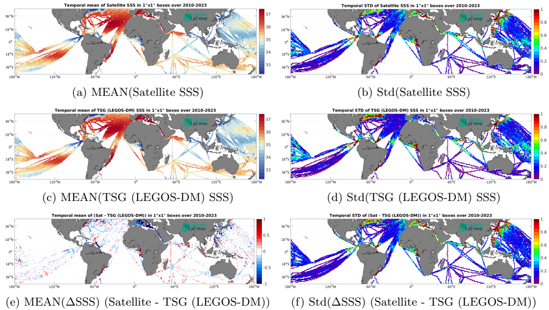
Figure 7: Temporal mean (left) and Std (right) of SSS from SMOS SSS L3 v335 - Monthly - 25 km (CATDS-CPDC) (top), TSG (LEGOS-DM) (middle), and of \Delta SSS (Satellite - TSG (LEGOS-DM)). Only match-up pairs are used to generate these maps.
