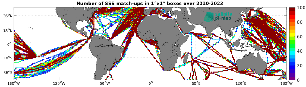
Figure 5: Number of SSS match-ups between TSG (LEGOS-DM) SSS and the SMOS SSS L3 v335 - Monthly - 25 km (CATDS-CPDC) SSS product for the Mid-Low Latitudes 45N-45S Pi-MEP region over 1^\circ \times 1^\circ boxes and for the full satellite product period.
