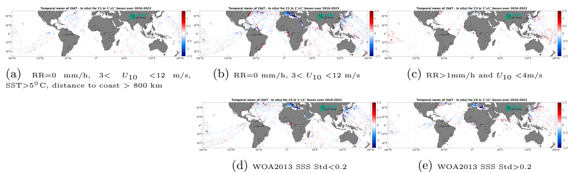
Figure 14: Temporal mean gridded over spatial boxes of size 1^\circ \times 1^\circ of \Delta\text{SSS} (SMOS SSS L3 v335 - Monthly - 25 km (CATDS-CPDC) - TSG (LEGOS-DM)) for 5 different subdatasets corresponding to: RR=0 mm/h, 3 < U_{10} < 12 m/s, SST > 5°C, distance to coast > 800 km (a), RR=0 mm/h, 3 < U_{10} < 12 m/s (b), RR > 1mm/h and U_{10} < 4 m/s (c), WOA2013 SSS Std < 0.2 (d), WOA2013 SSS Std > 0.2 (e).
