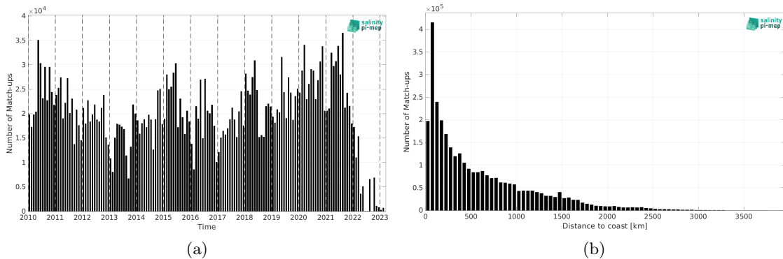
Figure 2: Number of match-ups between TSG (LEGOS-DM) and SMOS SSS L3 v335 - Monthly - 25 km (CATDS-CPDC) SSS as a function of time (a) and as function of the distance to coast (b) over the Mid-Low Latitudes 45N-45S Pi-MEP region and for the full satellite product period.
