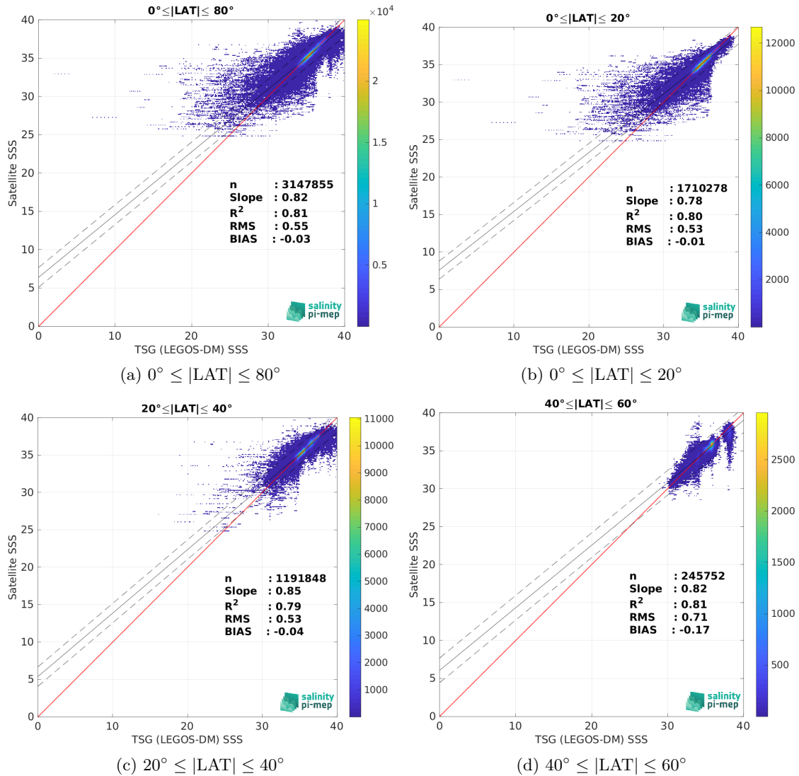
Figure 10: Contour maps of the concentration of SMOS SSS L3 v335 - Monthly - 25 km (CATDS-CPDC) SSS (y-axis) versus TSG (LEGOS-DM) SSS (x-axis) at match-up pairs for different latitude bands. For each plot, the red line shows x=y . The black thin and dashed lines indicate a linear fit through the data cloud and the \pm 95\% confidence levels, respectively. The number match-up pairs n , the slope and R^2 coefficient of the linear fit, the root mean square (RMS) and the mean bias between satellite and in situ data are indicated for each latitude band in each plots.
