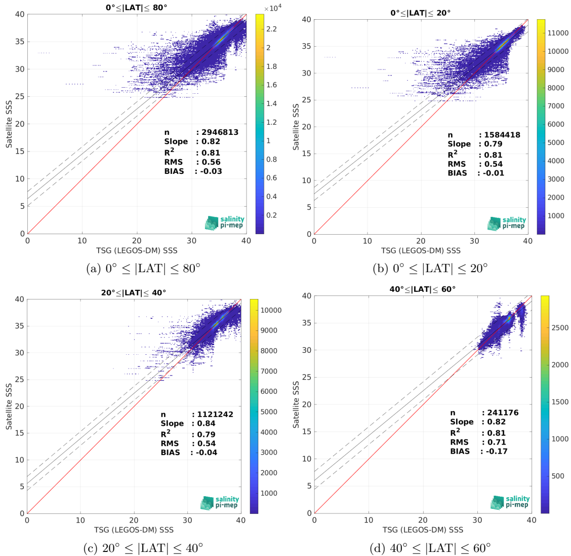
Figure 9: Contour maps of the concentration of SMOS SSS L3 v335 - Monthly - 25 km (CATDS-CPDC) SSS (y-axis) versus TSG (LEGOS-DM) SSS (x-axis) at match-up pairs for different latitude bands. For each plot, the red line shows x=y . The black thin and dashed lines indicate a linear fit through the data cloud and the \pm 95\% confidence levels, respectively. The number match-up pairs n , the slope and R^2 coefficient of the linear fit, the root mean square (RMS) and the mean bias between satellite and in situ data are indicated for each latitude band in each plots.
