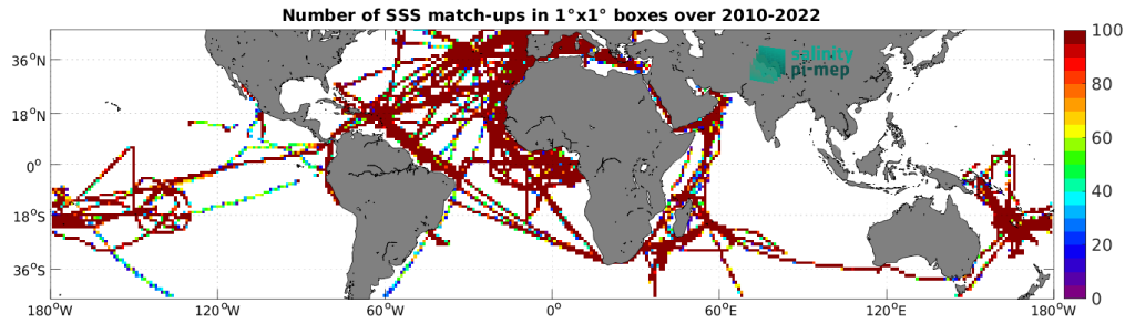
Figure 5: Number of SSS match-ups between TSG (GOSUD-Research-vessel) SSS and the SMOS SSS L3 v335 - Monthly - 25 km (CATDS-CPDC) SSS product for the Mid-Low Latitudes 45N-45S Pi-MEP region over 1^{\circ} \times 1^{\circ} boxes and for the full satellite product period.
