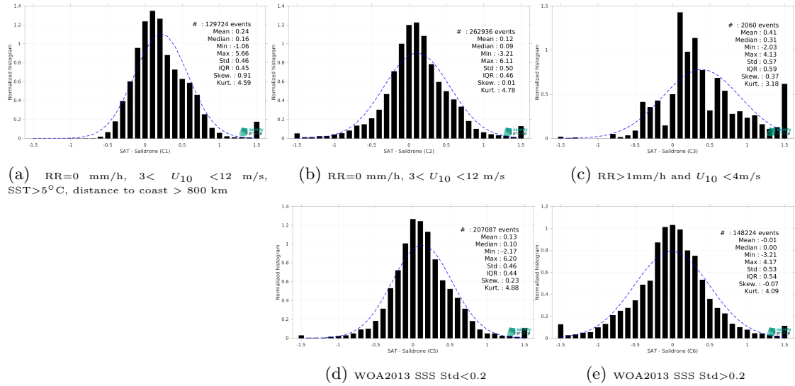
Figure 15: Normalized histogram of \Delta SSS (SMOS SSS L3 v335 - Monthly - 25 km (CATDS-CPDC) - Saldrone) for 5 different subdatasets corresponding to: RR=0 mm/h, 3 < U_{10} < 12 m/s, SST>5°C, distance to coast > 800 km (a), RR=0 mm/h, 3 < U_{10} < 12 m/s (b), RR>1mm/h and U_{10} < 4 m/s (c), WOA2013 SSS Std<0.2 (d), WOA2013 SSS Std>0.2 (e).
