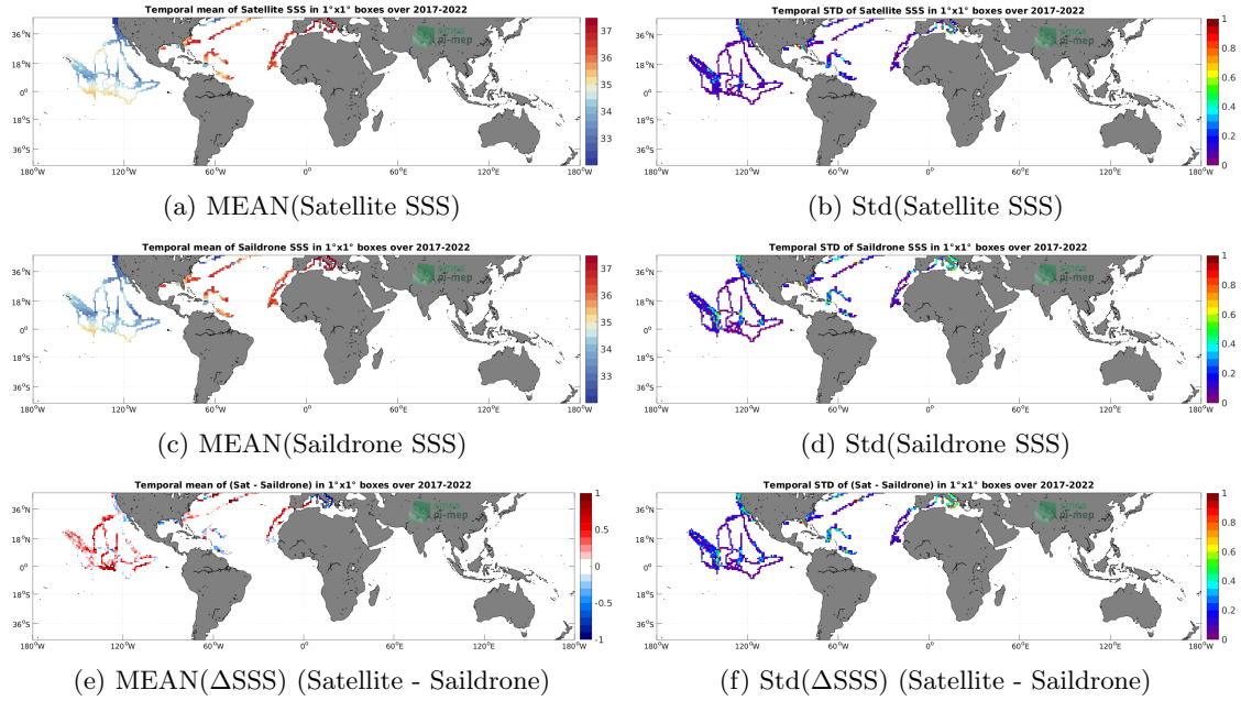
Figure 6: Temporal mean (left) and Std (right) of SSS from SMOS SSS L3 v335 - Monthly - 25 km (CATDS-CPDC) (top), Saildrone (middle), and of \Delta SSS (Satellite - Saildrone). Only match-up pairs are used to generate these maps.
