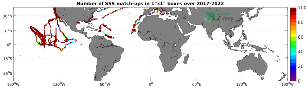
Figure 4: Number of SSS match-ups between Saildrone SSS and the SMOS SSS L3 v335 - Monthly - 25 km (CATDS-CPDC) SSS product for the Mid-Low Latitudes 45N-45S Pi-MEP region over 1^\circ \times 1^\circ boxes and for the full satellite product period.
