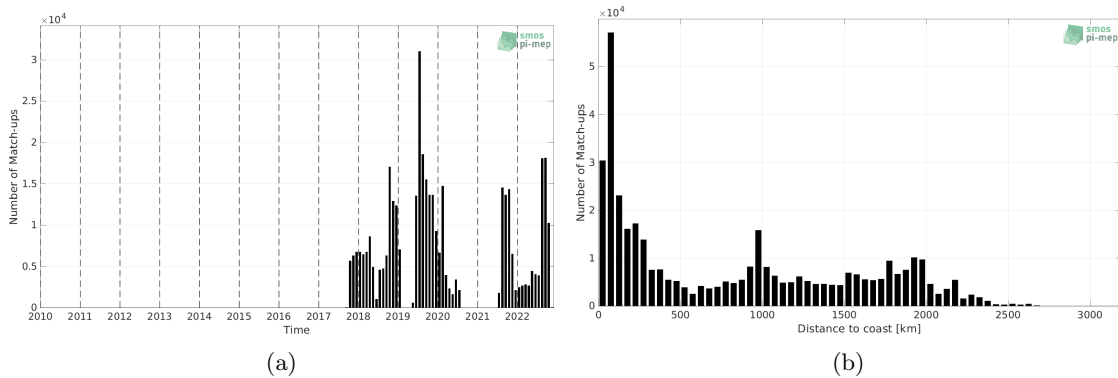
Figure 1: Number of match-ups between Saildrone and SMOS SSS L3 v335 - Monthly - 25 km (CATDS-CPDC) SSS as a function of time (a) and as function of the distance to coast (b) over the Mid-Low Latitudes 45N-45S Pi-MEP region and for the full satellite product period.
