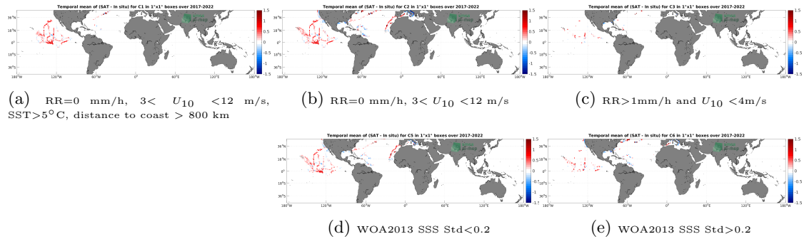
Figure 12: Temporal mean gridded over spatial boxes of size 1^\circ \times 1^\circ of \Delta SSS (SMOS SSS L3 v335 - Monthly - 25 km (CATDS-CPDC) - Saldrone) for 5 different subdatasets corresponding to:RR=0 mm/h, 3 < U_{10} < 12 m/s, SST >5^\circ C, distance to coast > 800 km (a), RR=0 mm/h, 3 < U_{10} < 12 m/s (b), RR >1 mm/h and U_{10} < 4 m/s (c), WOA2013 SSS Std <0.2 (d), WOA2013 SSS Std >0.2 (e).
