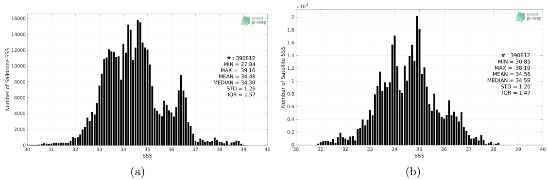
Figure 2: Histograms of SSS from Saildrone (a) and SMOS SSS L3 v335 - Monthly - 25 km (CATDS-CPDC) (b) considering all match-up pairs per bins of 0.1 over the Mid-Low Latitudes 45N-45S Pi-MEP region and for the full satellite product period.
