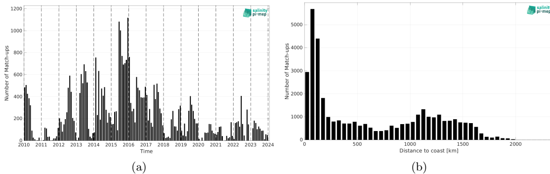
Figure 2: Number of match-ups between Marine mammals and SMOS SSS L3 v335 - Monthly - 25 km (CATDS-CPDC) SSS as a function of time (a) and as function of the distance to coast (b) over the Mid-Low Latitudes 45N-45S Pi-MEP region and for the full satellite product period.
