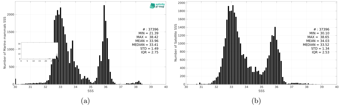
Figure 3: Histograms of SSS from Marine mammals (a) and SMOS SSS L3 v335 - Monthly - 25 km (CATDS-CPDC) (b) considering all match-up pairs per bins of 0.1 over the Mid-Low Latitudes 45N-45S Pi-MEP region and for the full satellite product period.
