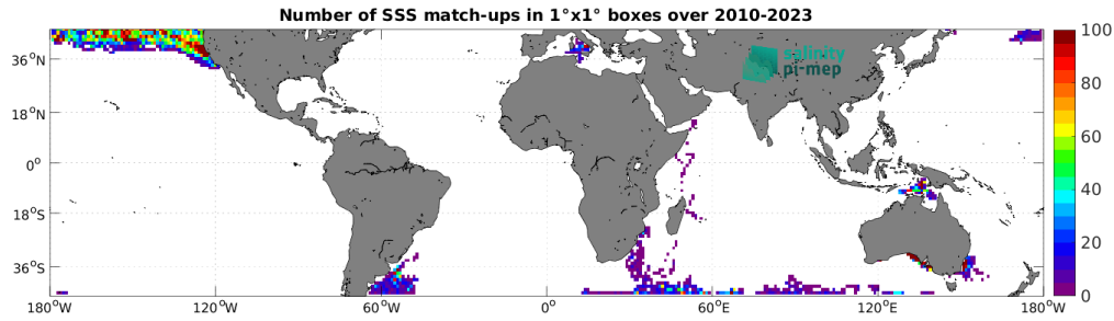
Figure 5: Number of SSS match-ups between Marine mammals SSS and the SMOS SSS L3 v335 - Monthly - 25 km (CATDS-CPDC) SSS product for the Mid-Low Latitudes 45N-45S Pi-MEP region over 1^\circ \times 1^\circ boxes and for the full satellite product period.
