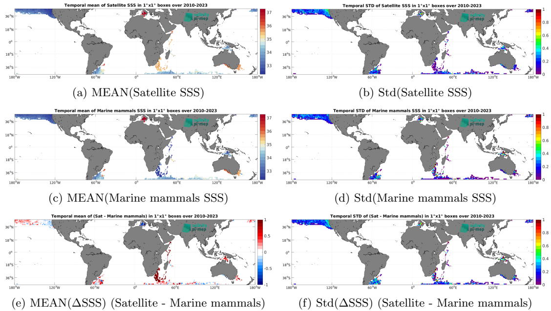
Figure 7: Temporal mean (left) and Std (right) of SSS from SMOS SSS L3 v335 - Monthly - 25 km (CATDS-CPDC) (top), Marine mammals (middle), and of \Delta SSS (Satellite - Marine mammals). Only match-up pairs are used to generate these maps.
