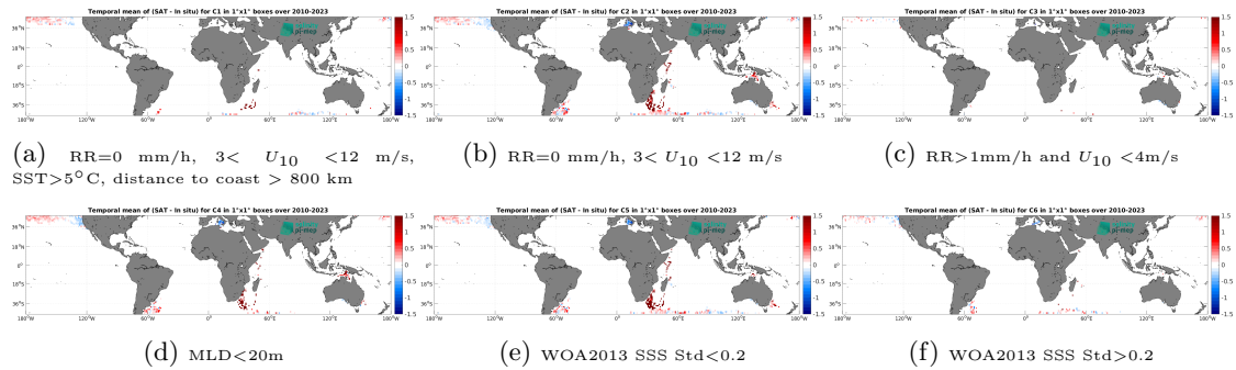
Figure 14: Temporal mean gridded over spatial boxes of size 1^\circ \times 1^\circ of \Delta SSS (SMOS SSS L3 v335 - Monthly - 25 km (CATDS-CPDC) - Marine mammals) for 6 different subdatasets corresponding to:RR=0 mm/h, 3 < U_{10} < 12 m/s, SST >5^\circ C, distance to coast > 800 km (a), RR=0 mm/h, 3 < U_{10} < 12 m/s (b), RR >1 mm/h and U_{10} < 4 m/s (c),MLD <20 m (d),WOA2013 SSS Std <0.2 (e),WOA2013 SSS Std >0.2 (f).
