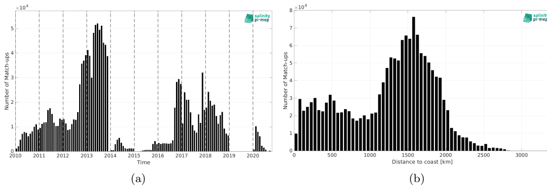
Figure 2: Number of match-ups between Surface drifters and SMOS SSS L3 v335 - Monthly - 25 km (CATDS-CPDC) SSS as a function of time (a) and as function of the distance to coast (b) over the Mid-Low Latitudes 45N-45S Pi-MEP region and for the full satellite product period.
