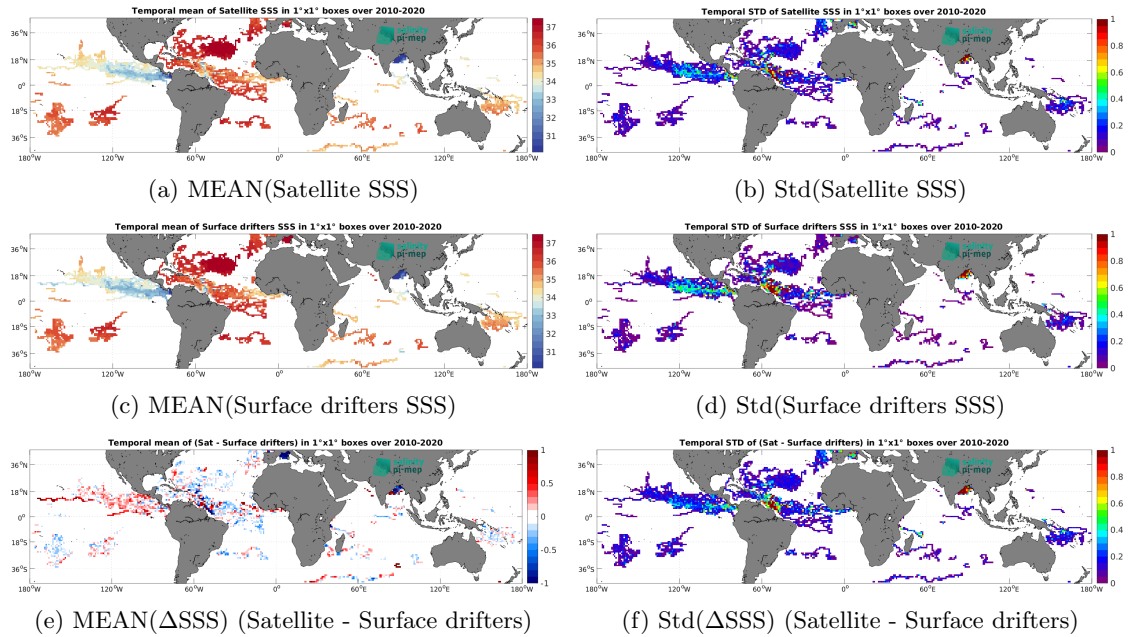
Figure 6: Temporal mean (left) and Std (right) of SSS from SMOS SSS L3 v335 - Monthly - 25 km (CATDS-CPDC) (top), Surface drifters (middle), and of \Delta SSS (Satellite - Surface drifters). Only match-up pairs are used to generate these maps.
